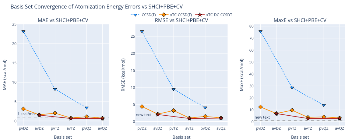
Figure 1: Basis set convergence of atomization energy errors vs SHCI+PBE+CV. [interactive]
