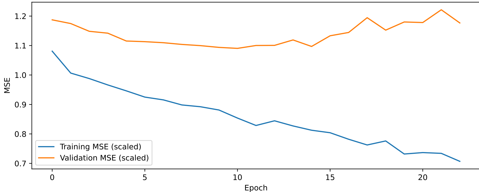
selected_lstm
