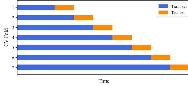
Fig. 8. The applied time series cross-validation approach.
