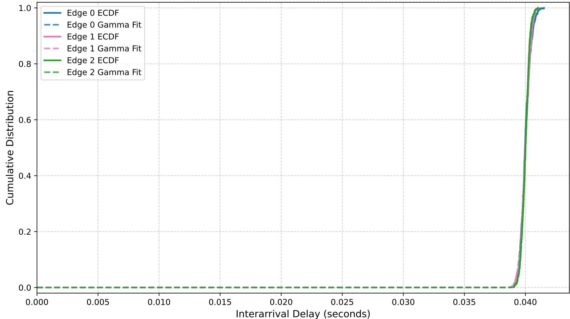
Empirical Distribution of Interarrival Delays in the Physical System
