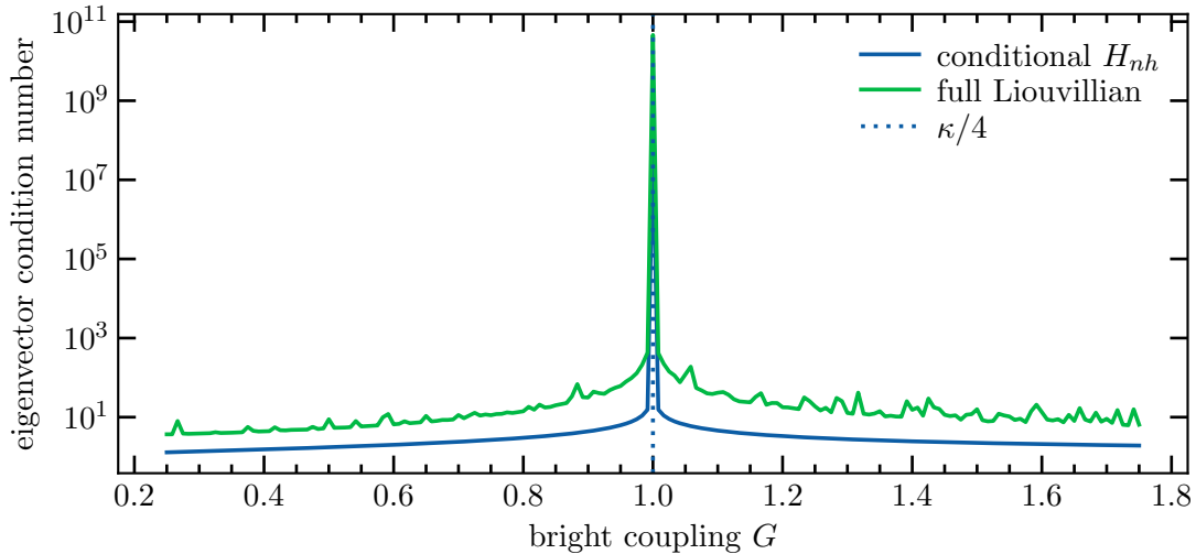
Conditional and Liouvillian defectiveness
