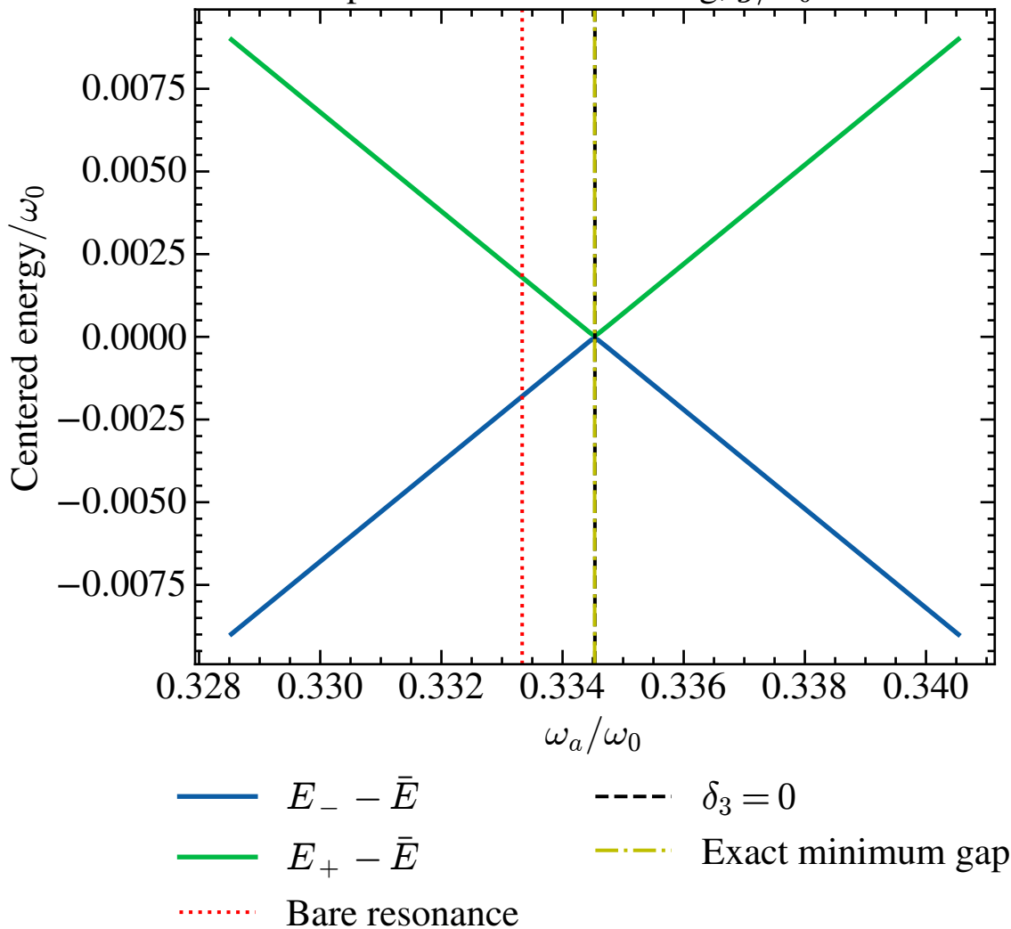
Three-photon avoided crossing, g/\omega_0 = 0.020
