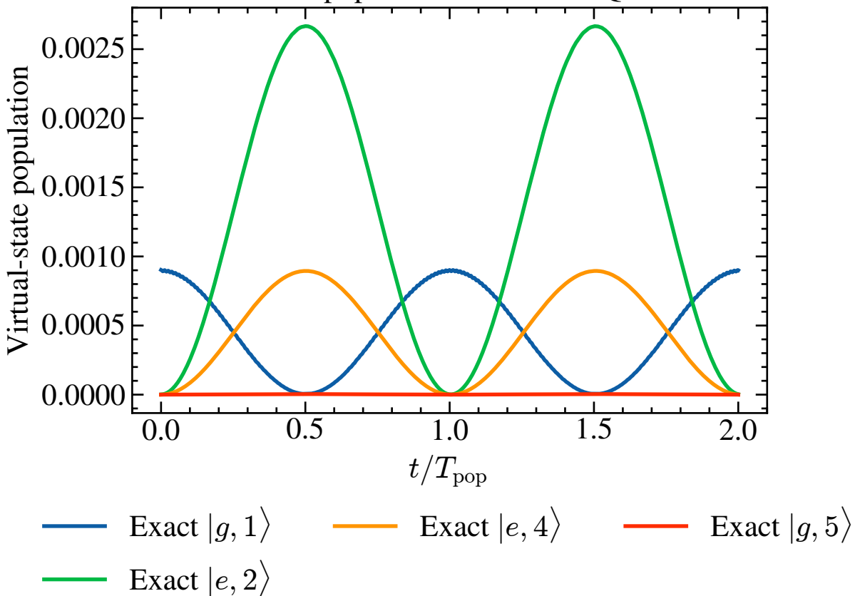
Virtual populations in the full QRM
