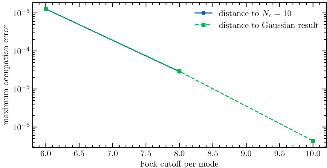
QuTiP cutoff convergence
