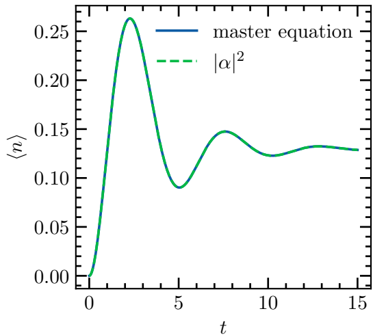
Driven vacuum cavity
