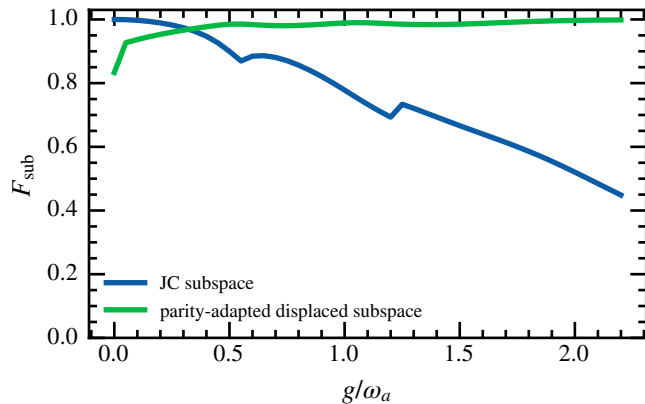
(c) Displaced-oscillator doublets
