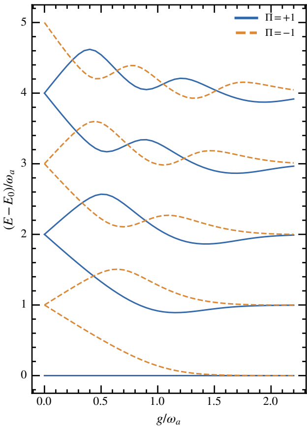
(a) Exact parity-resolved spectrum
