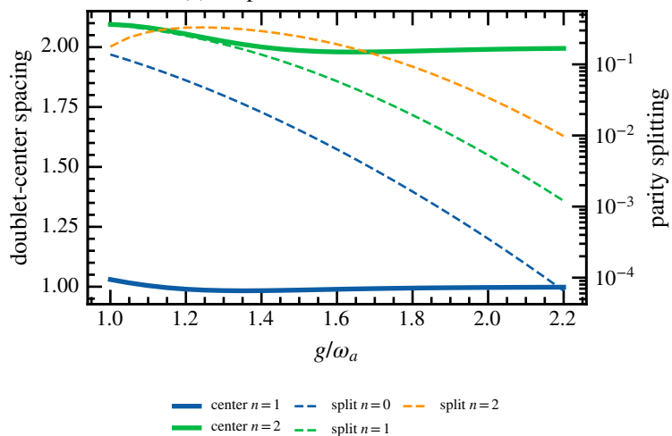
(c) Displaced-oscillator doublets
