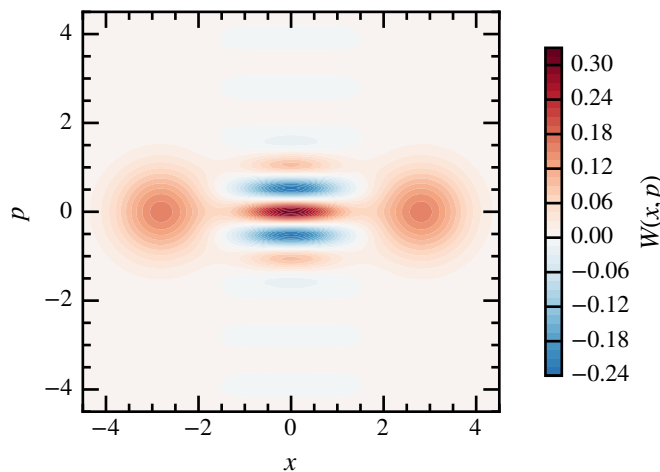
(e) Conditioned on |g\rangle
