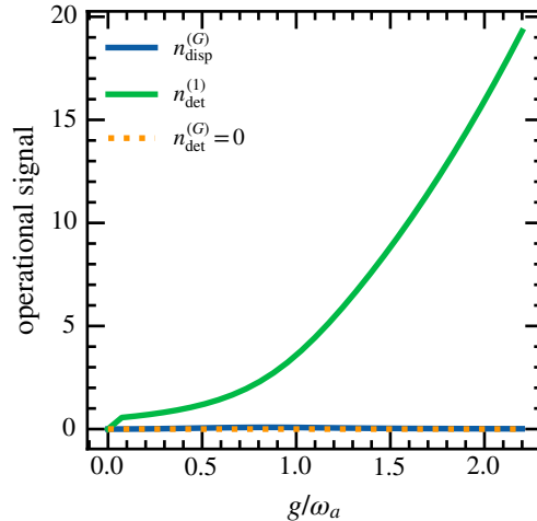
(e) Conditioned on |g\rangle
