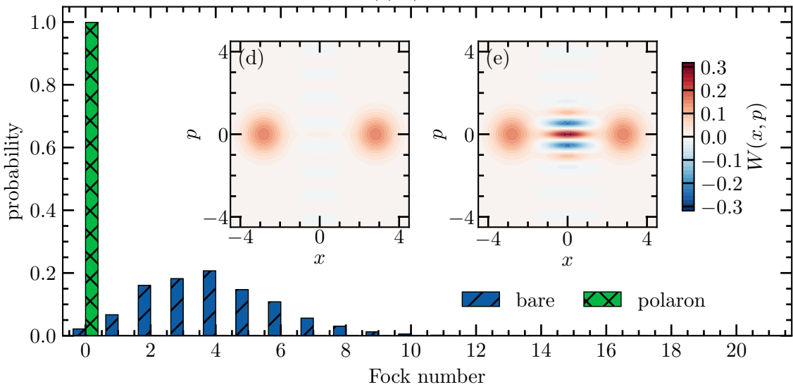
(c) g/\omega_a = 2
