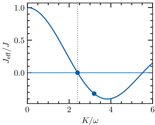
(a) Bessel-renormalized tunnelling
