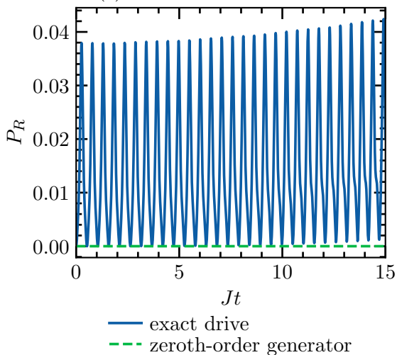
(c) Near coherent destruction
