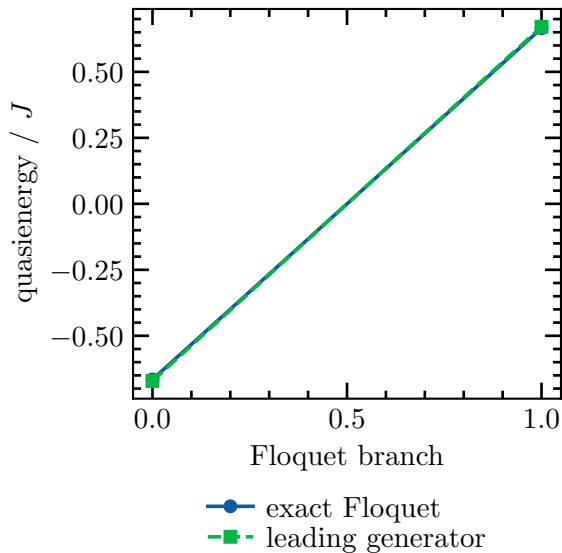
(a) Quasienergy-zone comparison
