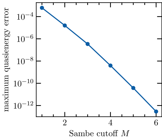
(b) Harmonic-cutoff convergence
