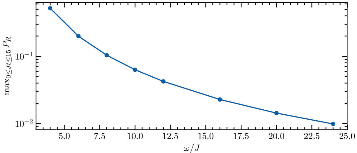
Finite-frequency motion at the first Bessel zero
