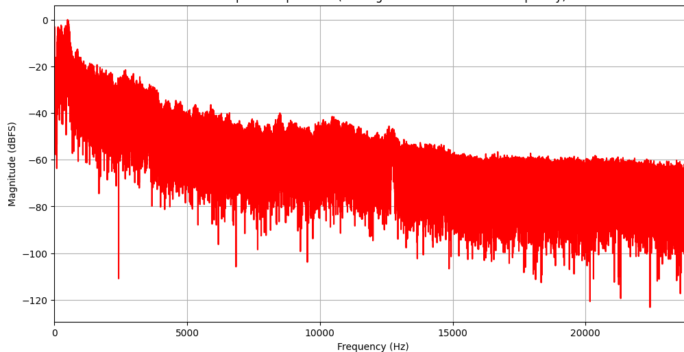
2. FFT Amplitude Spectrum (Finding the Dominant Noise Frequency)
