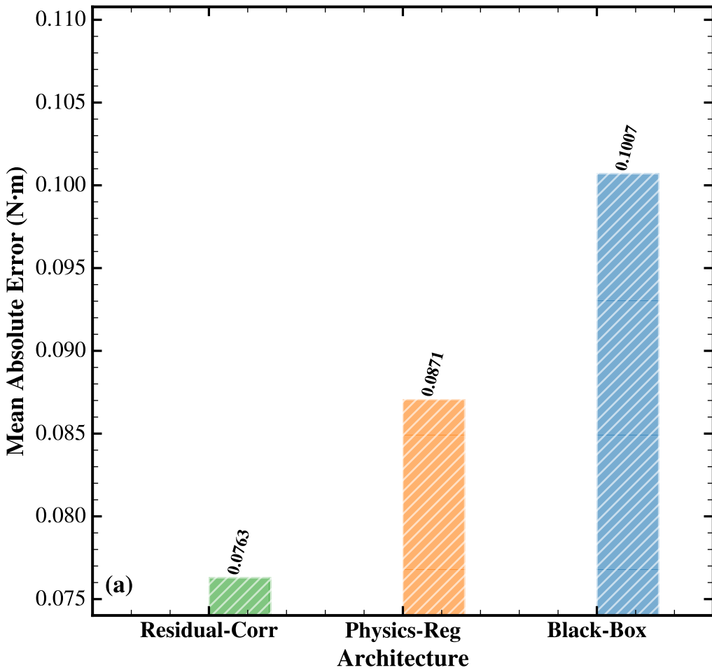
(a) MAE
