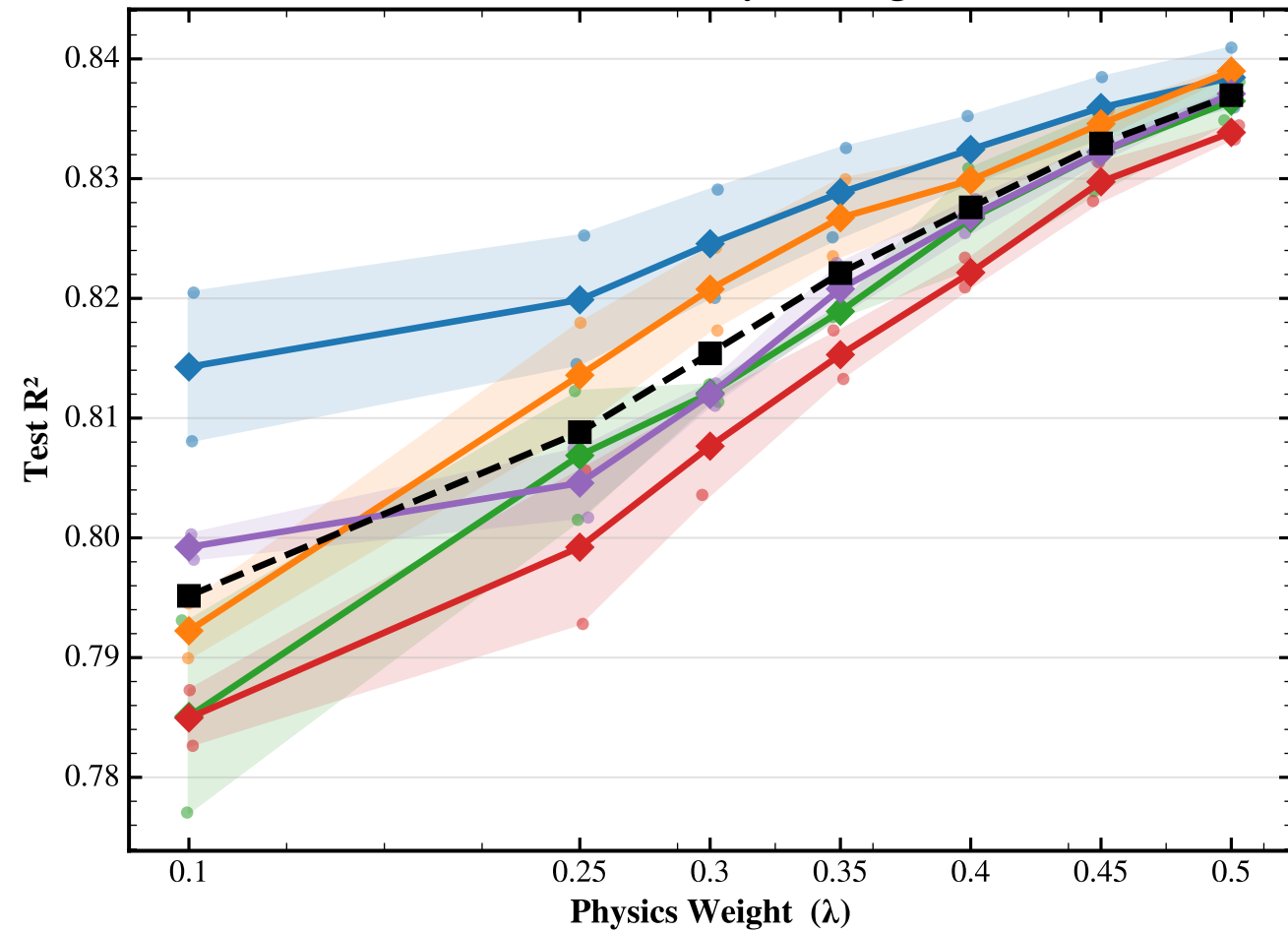
(b) Test R 2 vs Physics Weight
