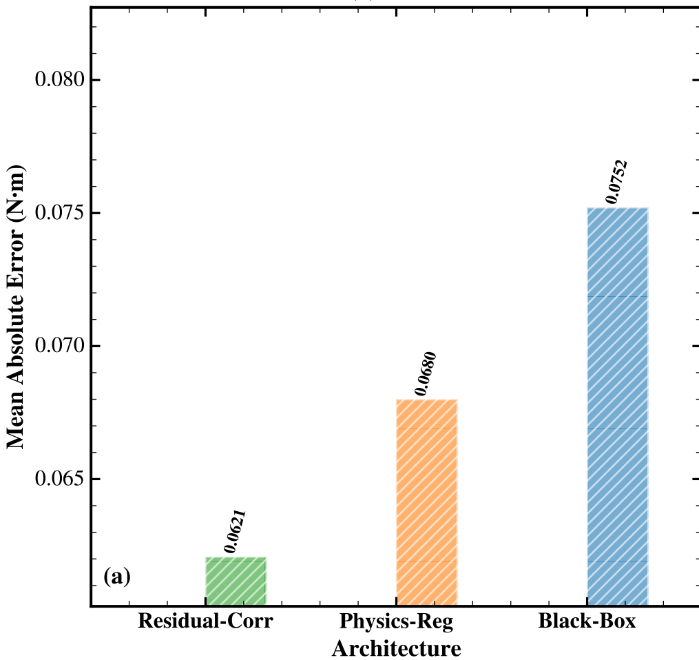
(a) MAE
