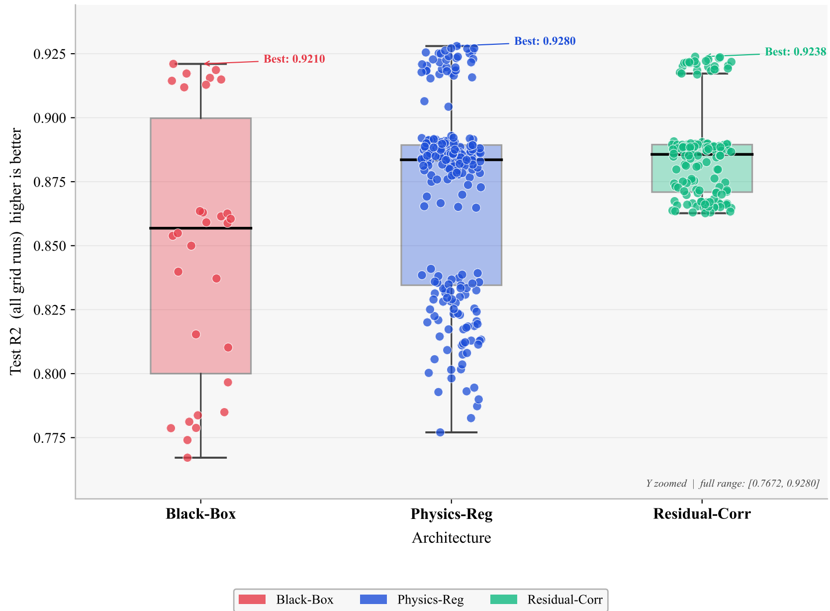
Test R2 distribution
