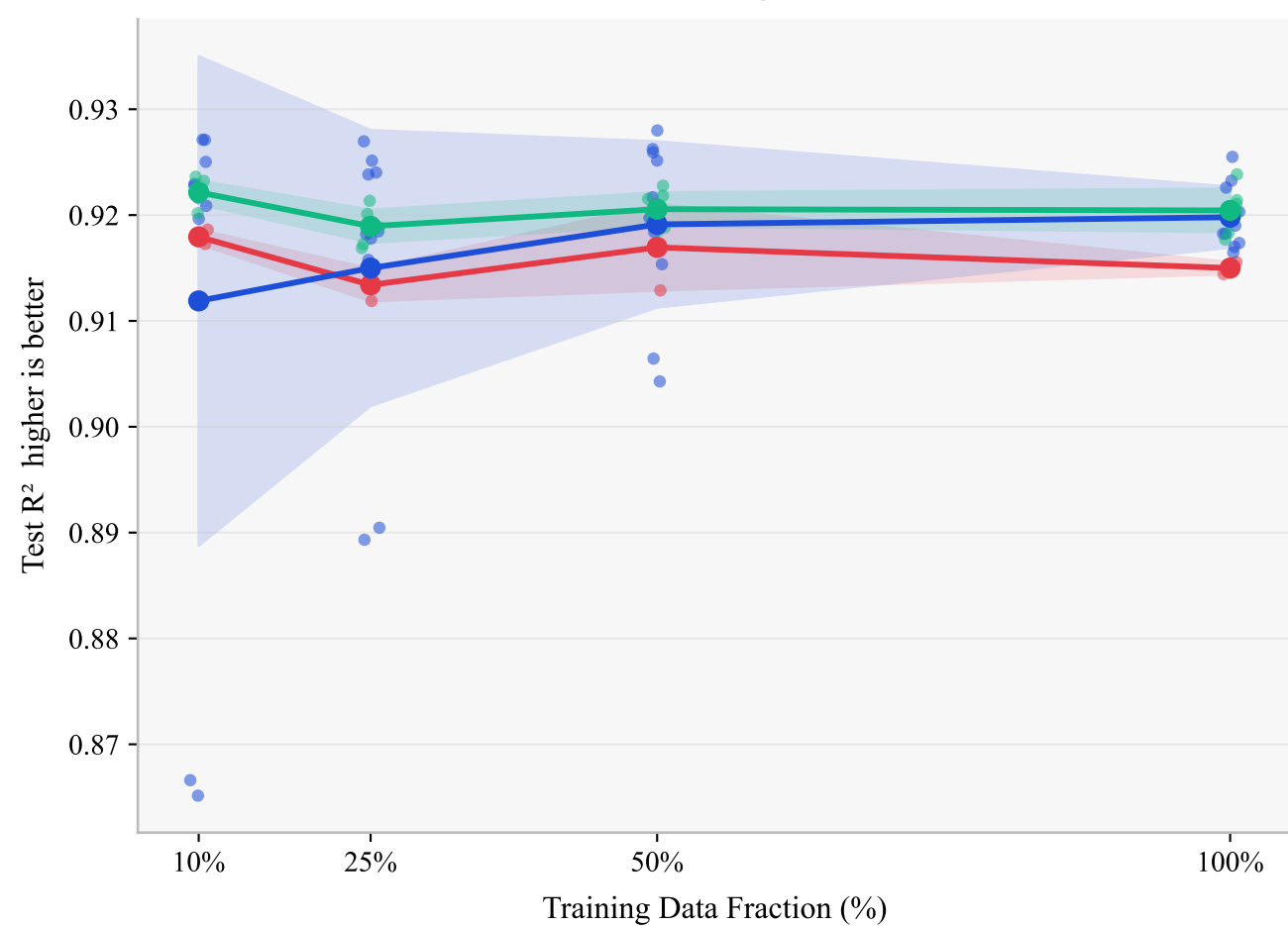
(b) Test R^2 vs Training Data Fraction
