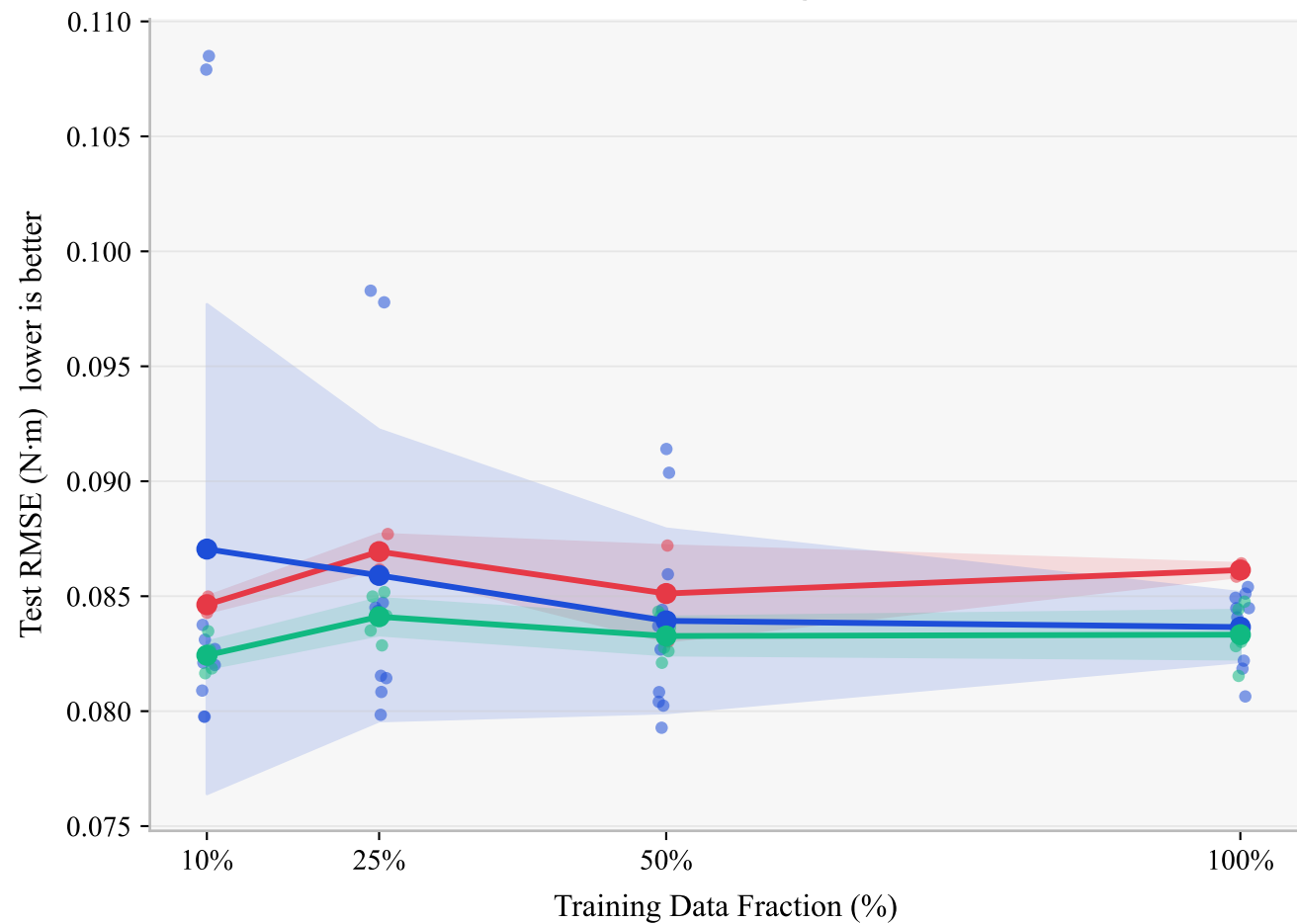
(a) Test RMSE vs Training Data Fraction
