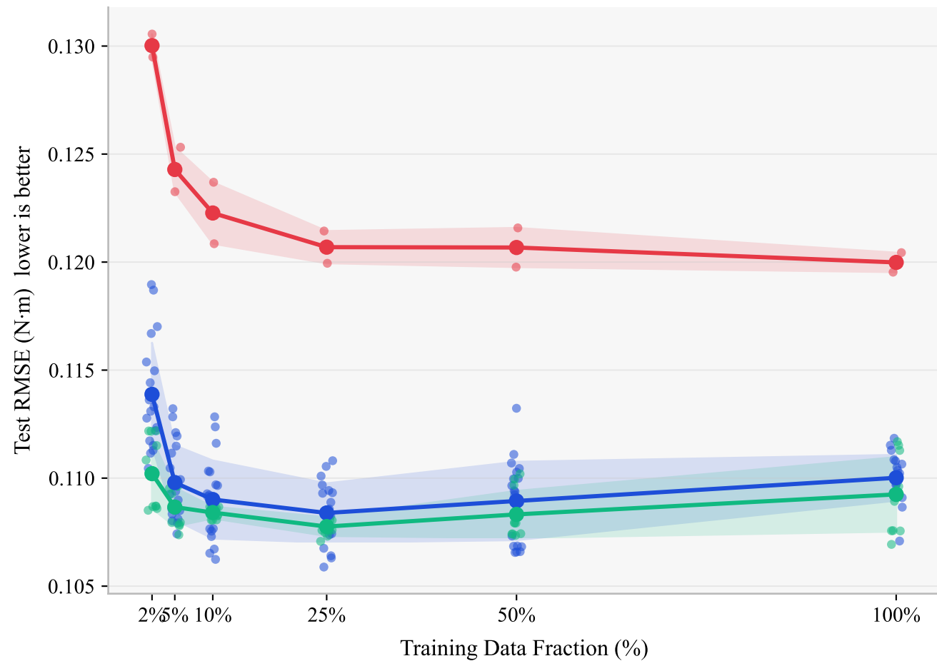
(a) Test RMSE vs Training Data Fraction
