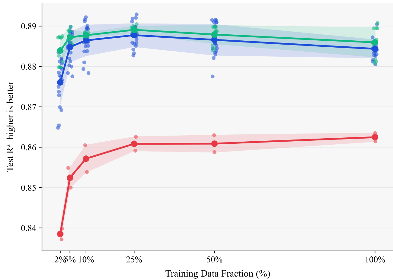
(b) Test R^2 vs Training Data Fraction
