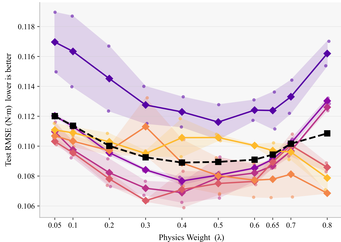
(a) Test RMSE vs Physics Weight ( \lambda )
