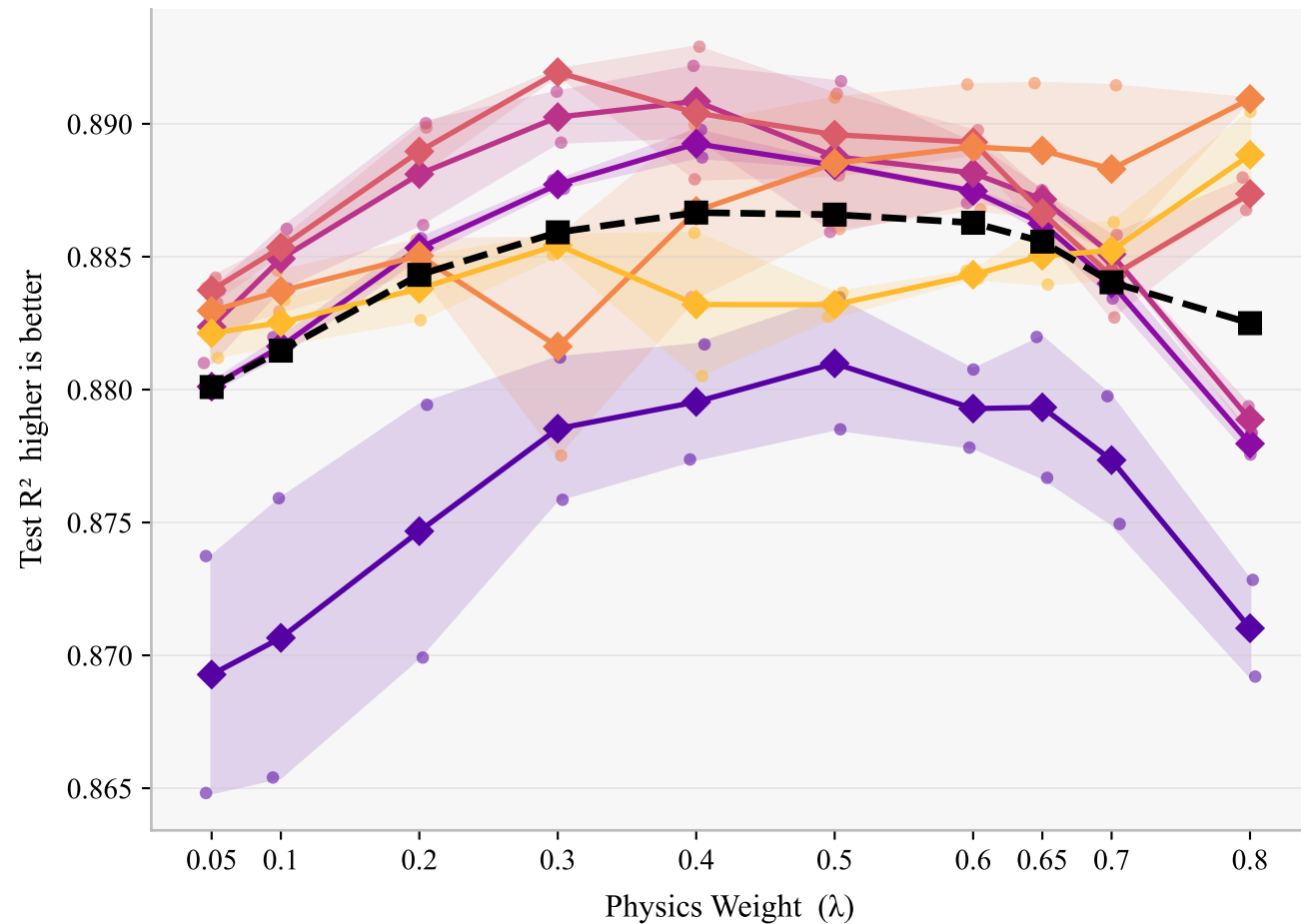
(b) Test R^2 vs Physics Weight ( \lambda )
