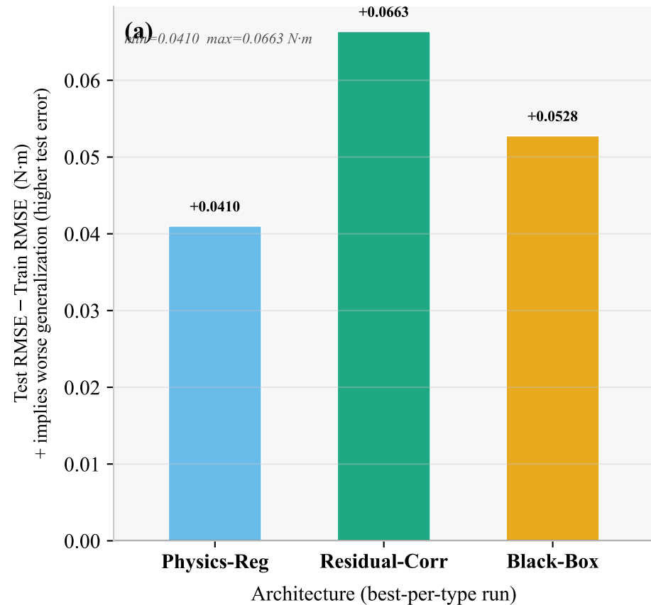
Generalization gap — pooled RMSE
