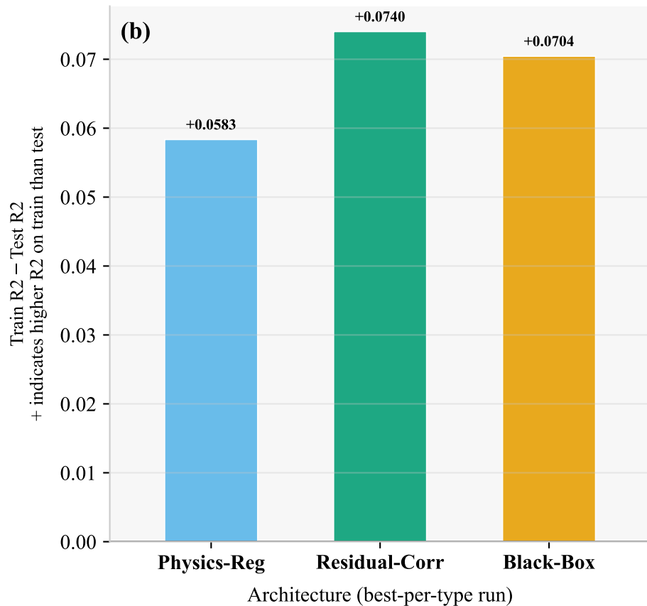
Generalization gap — R2 overall
