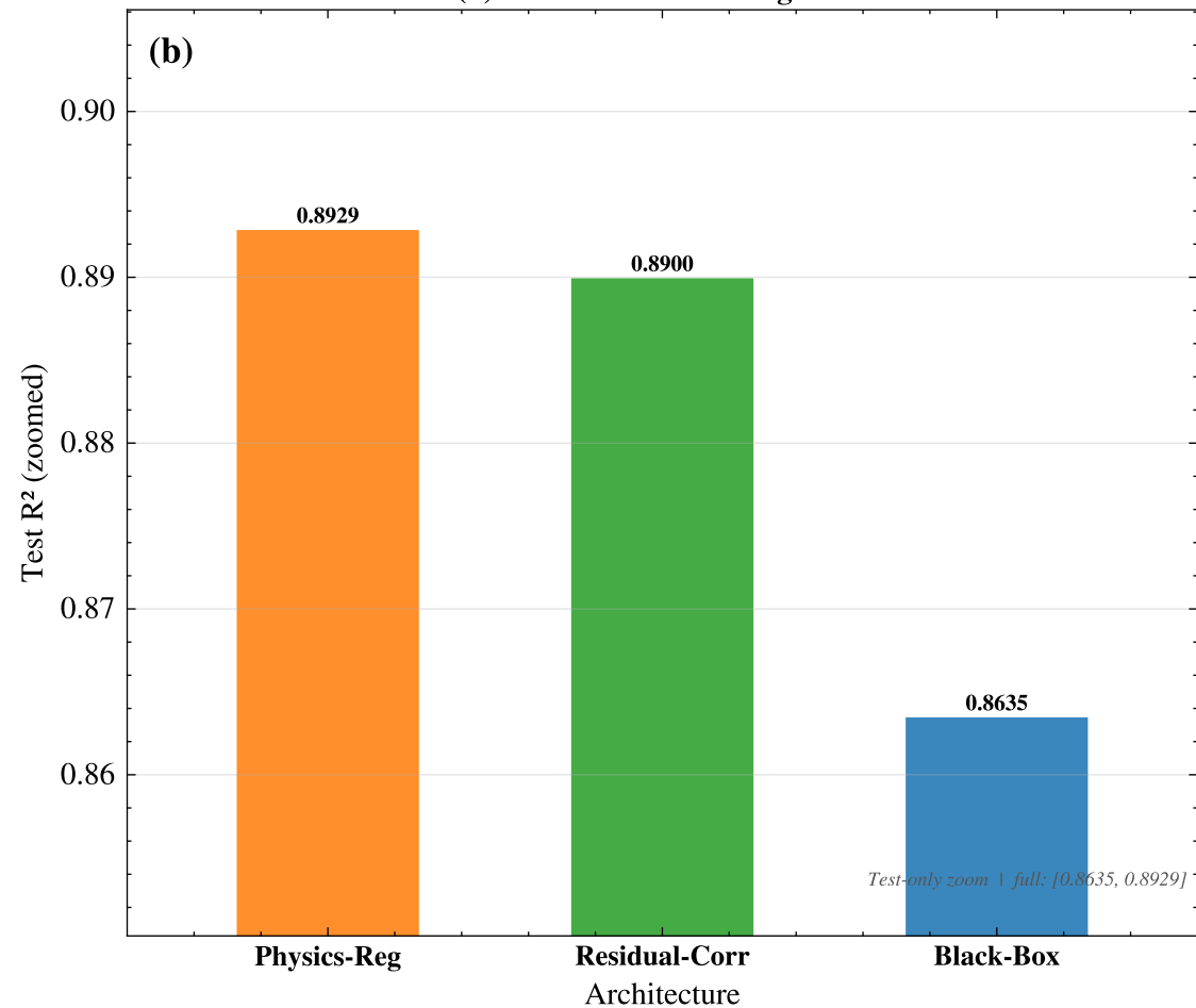
(b) Test R^2 overall -- magnified
