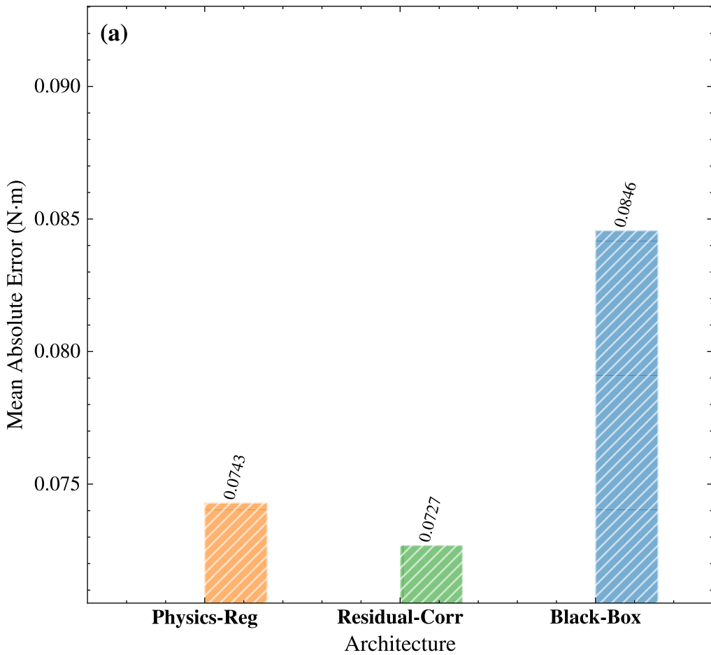
(a) MAE
