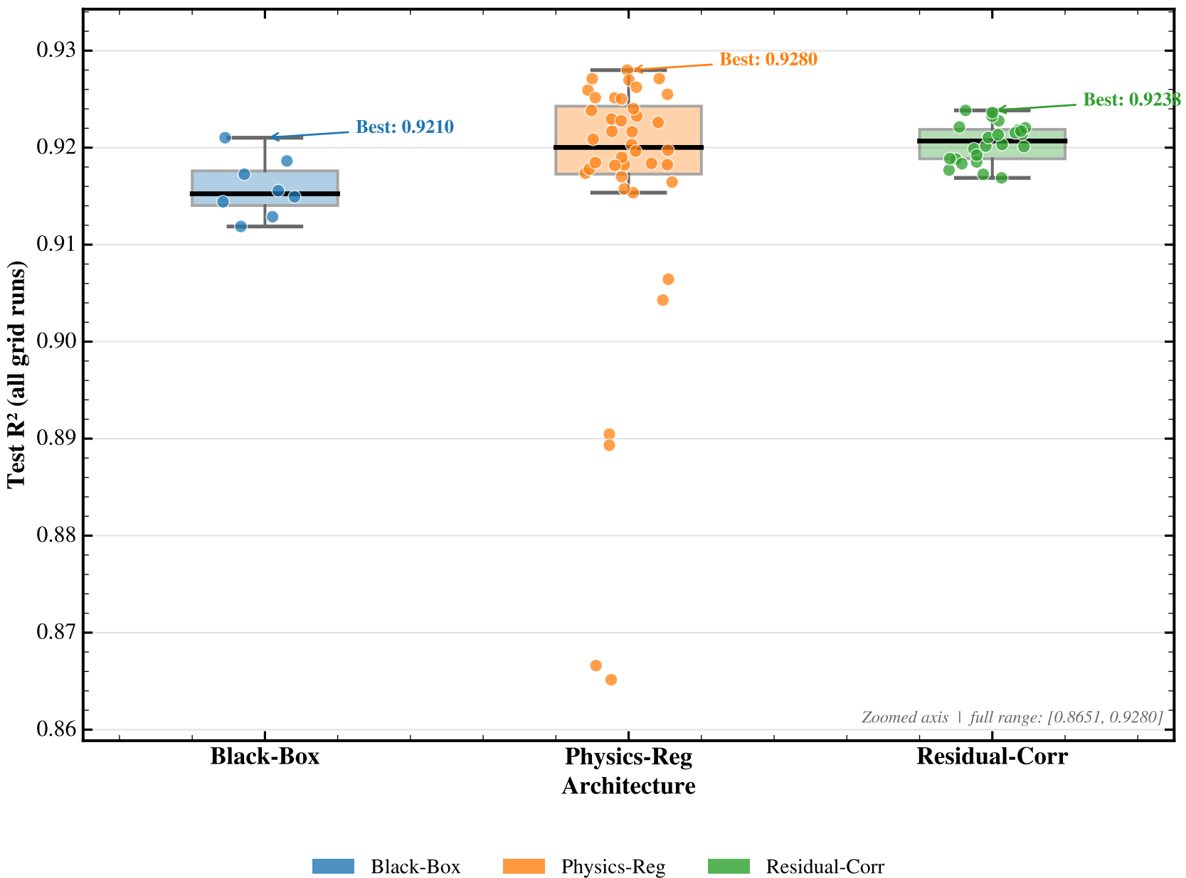
Test R 2 Distribution
