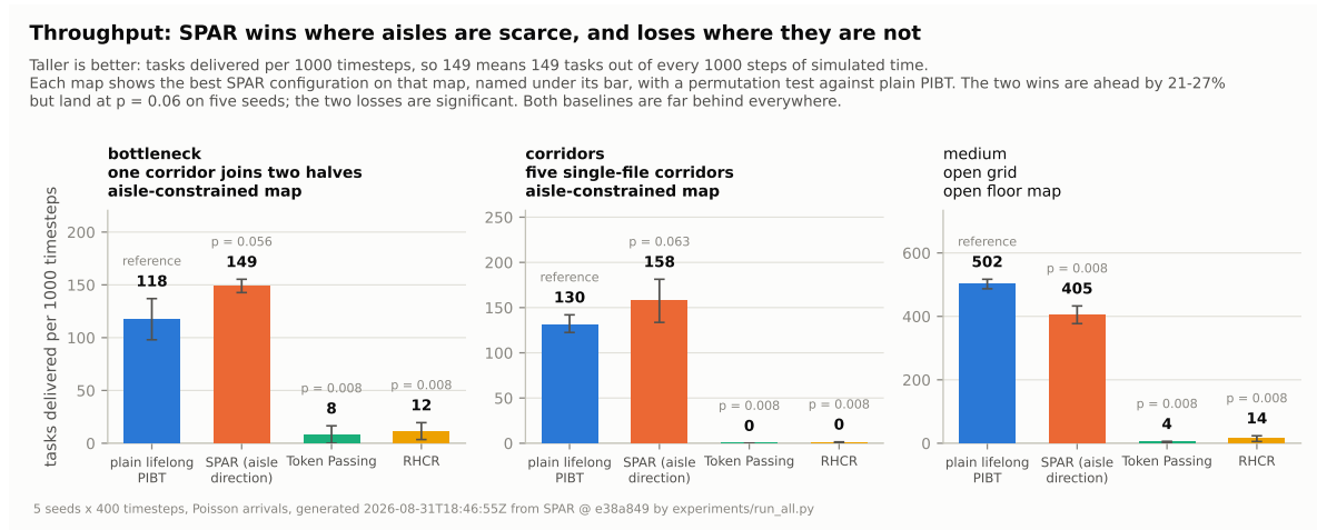
Figure 2: Throughput on the three maps the baseline suite covers. Both baselines are the two short bars on every panel.
