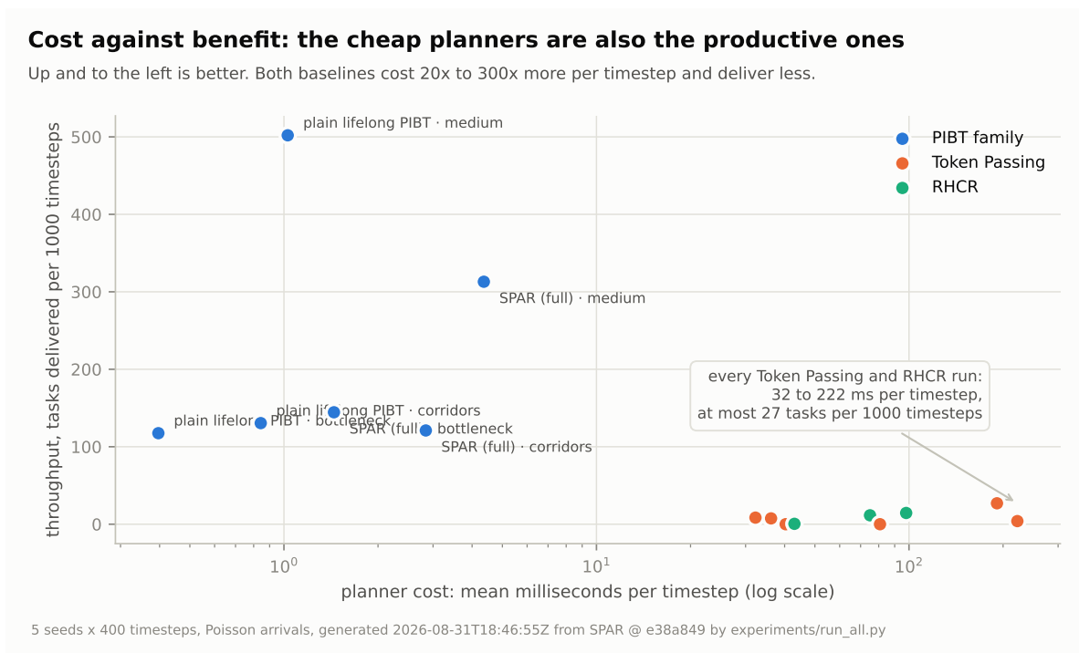
Figure 4: Planner cost against what it delivers; up and to the left is better. Note the log scale on cost.
