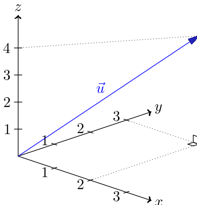
Figure 1: \vec{u} = [2, 3, 4]
