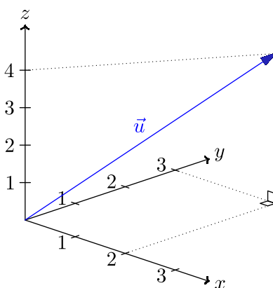
Figur 3.1: \vec{u} = [2, 3, 4]
