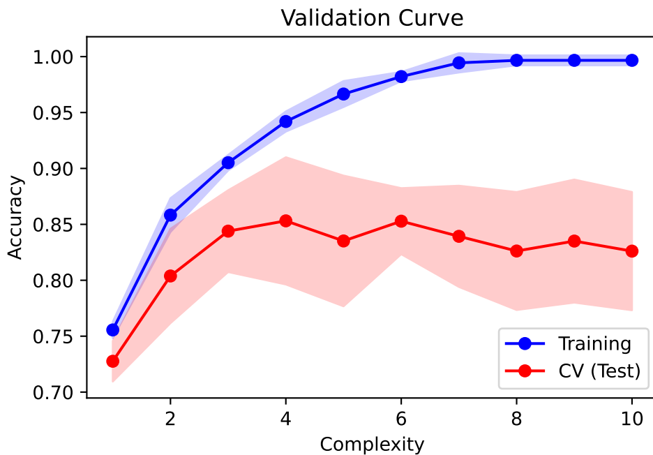
Figure 8.7: Validation curve, random forest
