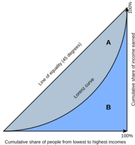
Figure 7.4: Lorenz curve
