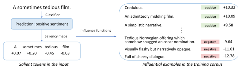
Figure 4.11: Han, Wallace, and Tsvetkov (2020)
