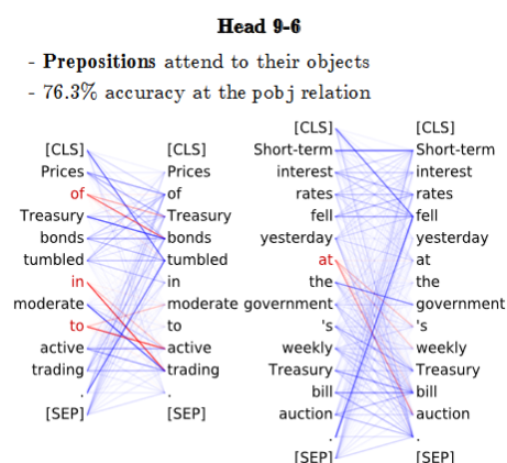
Figure 4.13: Clark et al. (2019)
