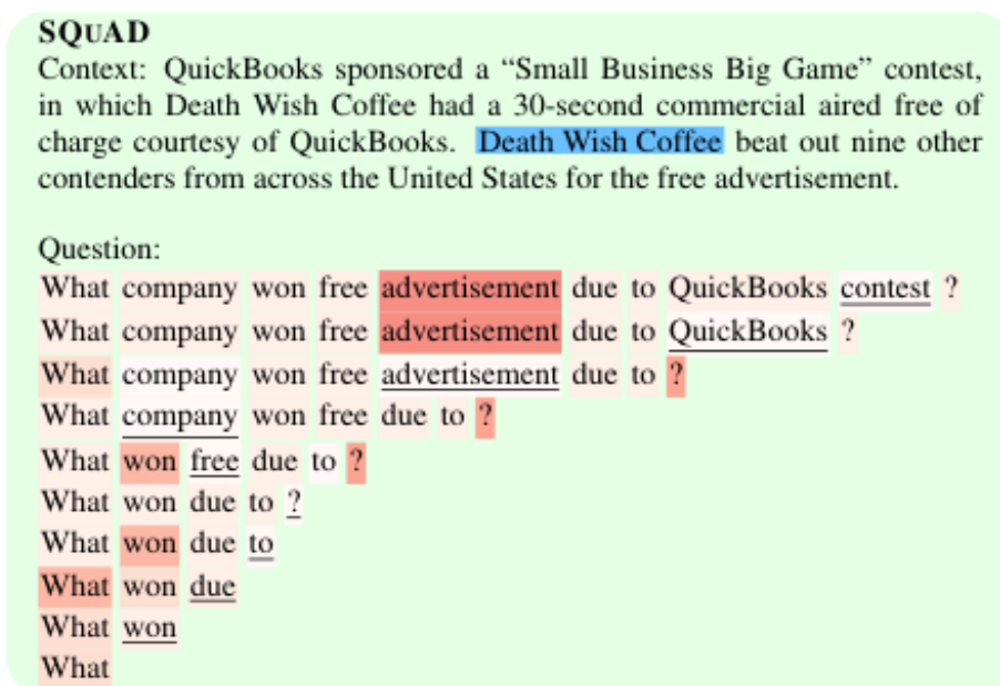
Figure 4.12: Sun et al. (2021)
