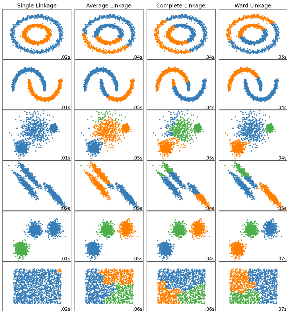
Figure 3.1: sklearn documentation
