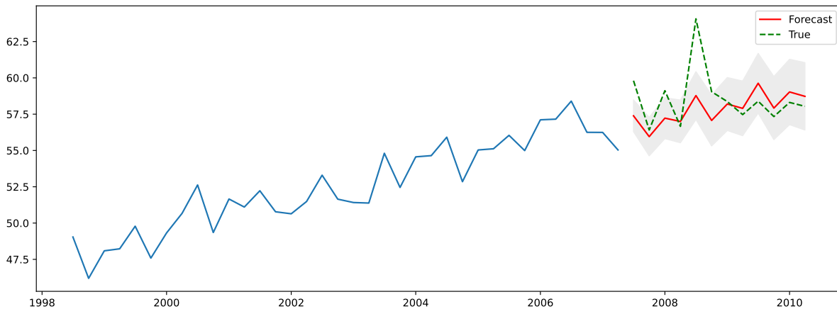
Figure 6.8: ARIMA forecasts
