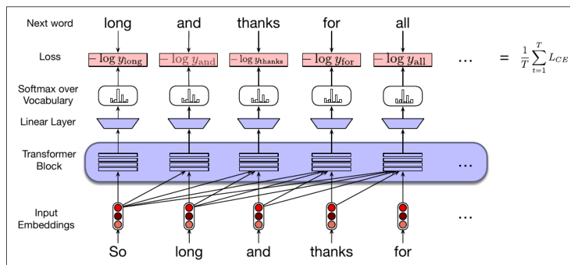
Figure 4.9: Jurafsky and Martin (2025)
