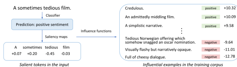
Figure 4.12: Han, Wallace, and Tsvetkov (2020)
