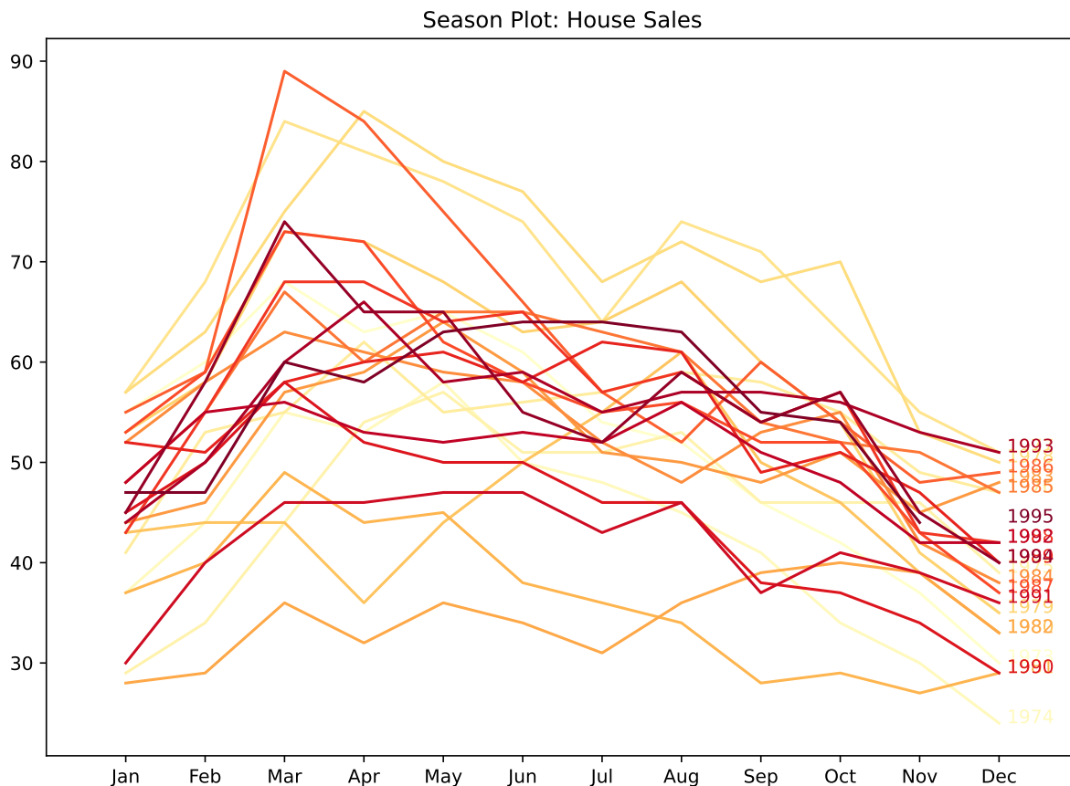
Figure 6.1: Season plot of housing sales
