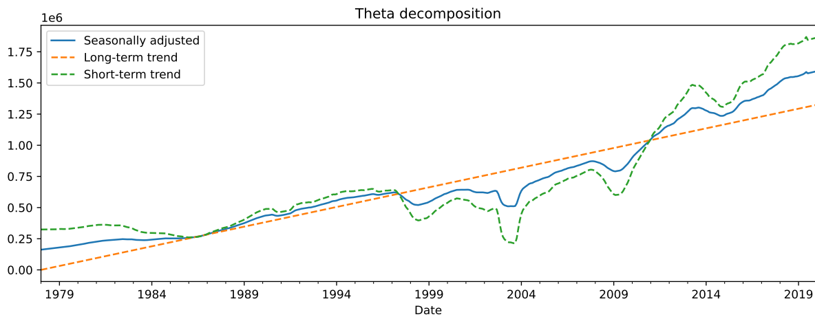
Figure 6.12: Theta decomposition
