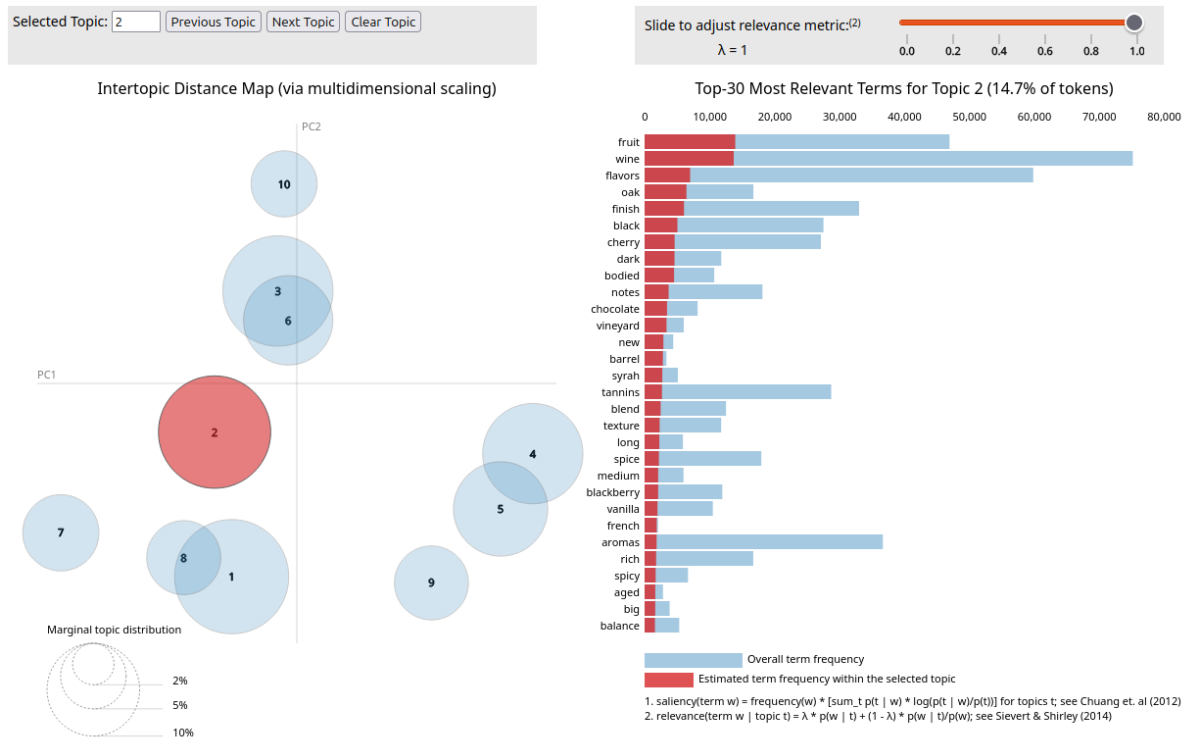
Figure 4.11: LDA visualisation
