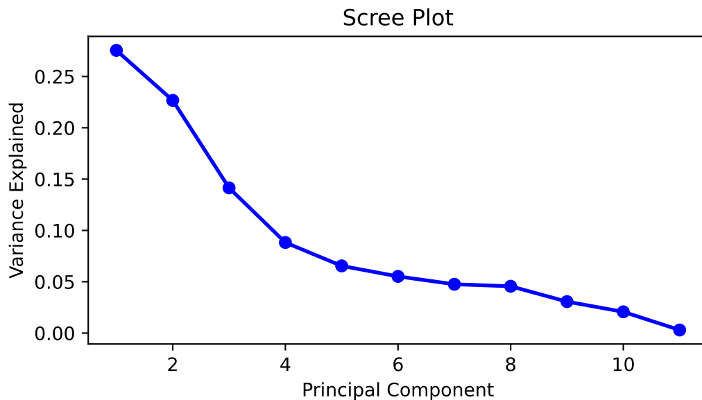
Figure 3.1: Scree plot
