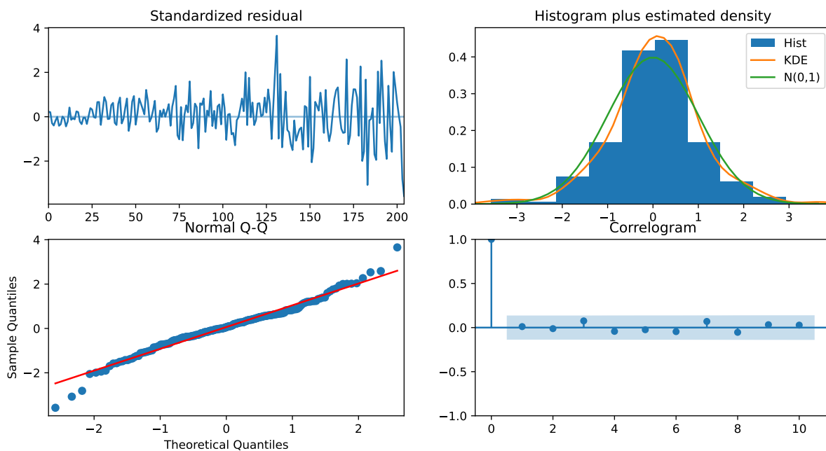
Figure 6.7: ARIMA residual diagnostics
