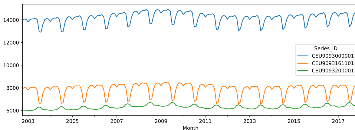
Figure 6.15: Series from bottom right corner of heatmap
