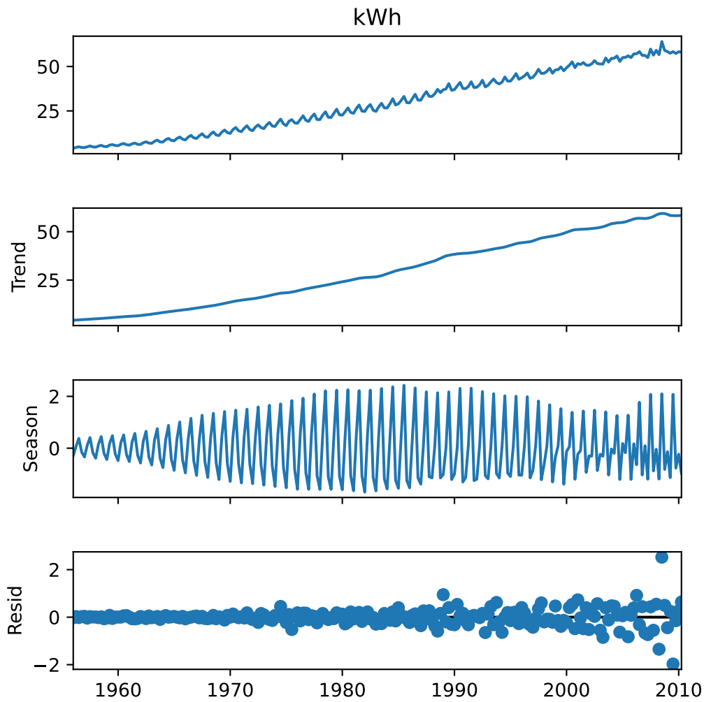
Figure 6.4: STL decomposition, electricity data
