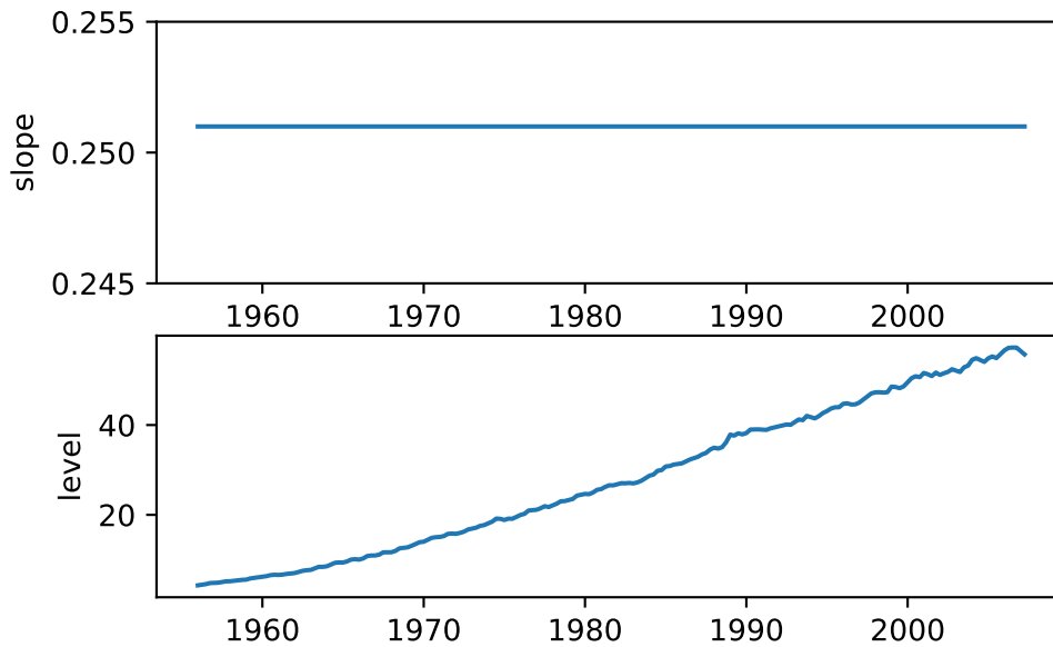
Figure 6.11: ETS trend and level components
