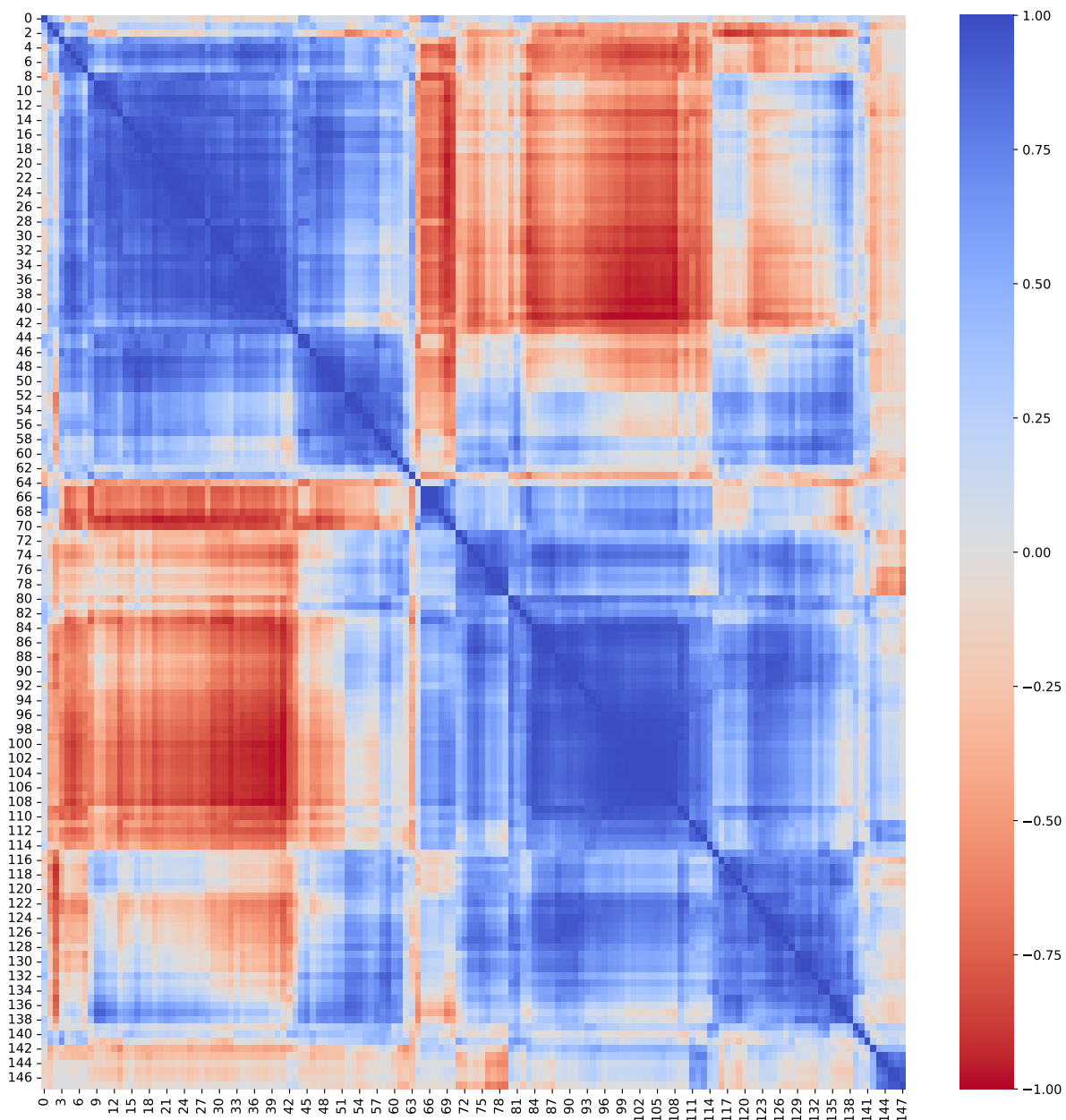
Figure 6.13: Heatmap of correlation matrix
