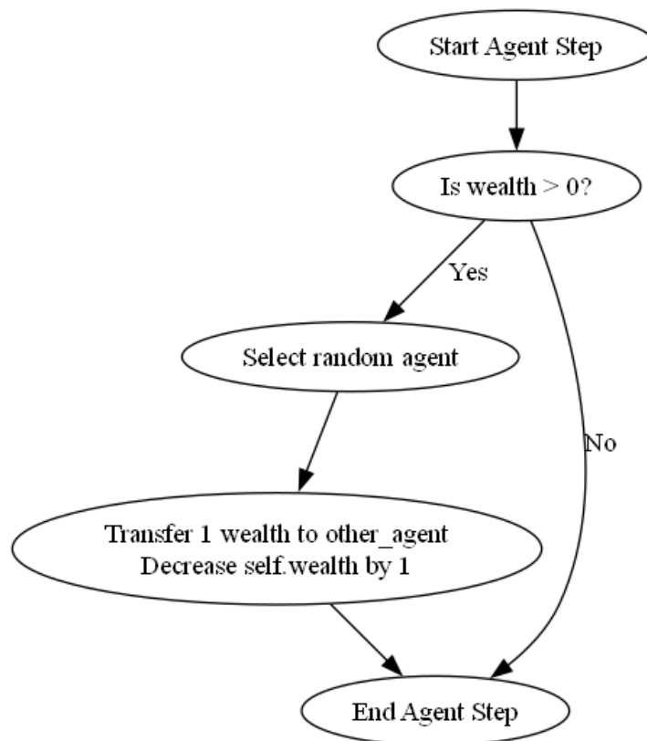
Figure 7.3: Agent trajectory
