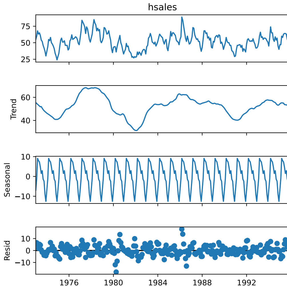
Figure 6.3: Additive decomposition
