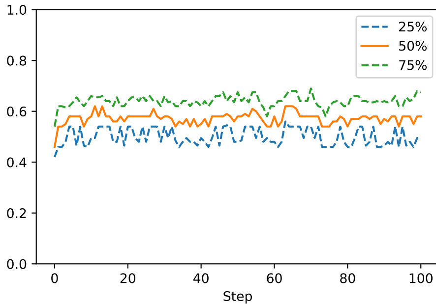
Figure 7.5: Evolution of Gini coefficient
