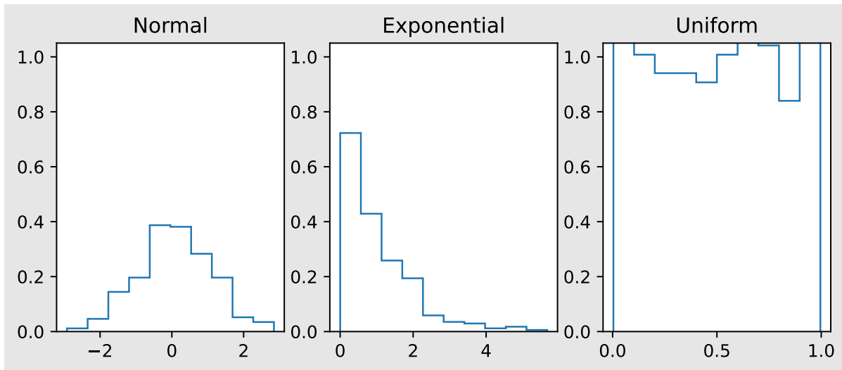
Figure 7.2: Histogram of random variables
