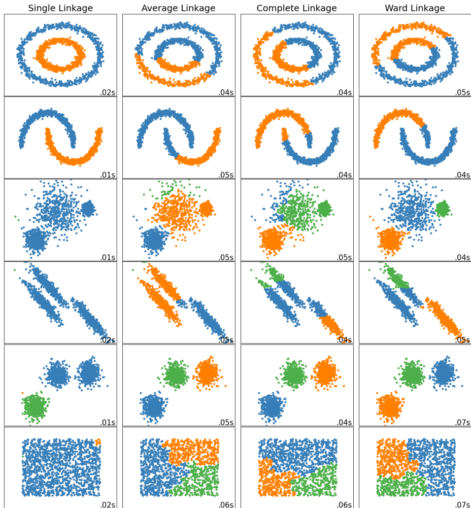
Figure 3.2: sklearn documentation
