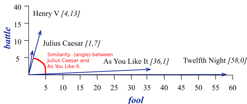
Figure 4.3: Jurafsky and Martin (2025)
