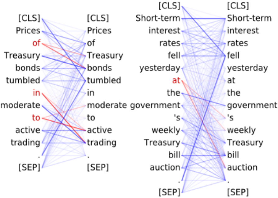
Figure 4.14: Clark et al. (2019)
