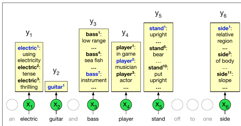
Figure 4.10: Jurafsky and Martin (2025)
