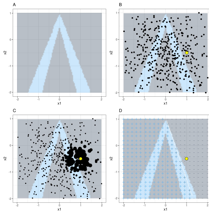
Figure 8.9: LIME
