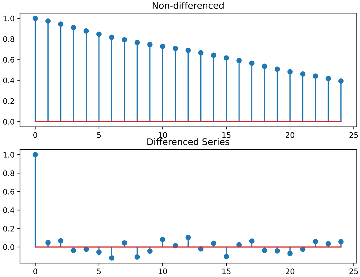
Figure 6.6: ACF, before and after differencing
