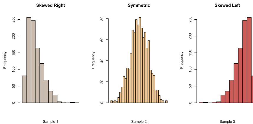
Figure 2.1: Sample Histograms
