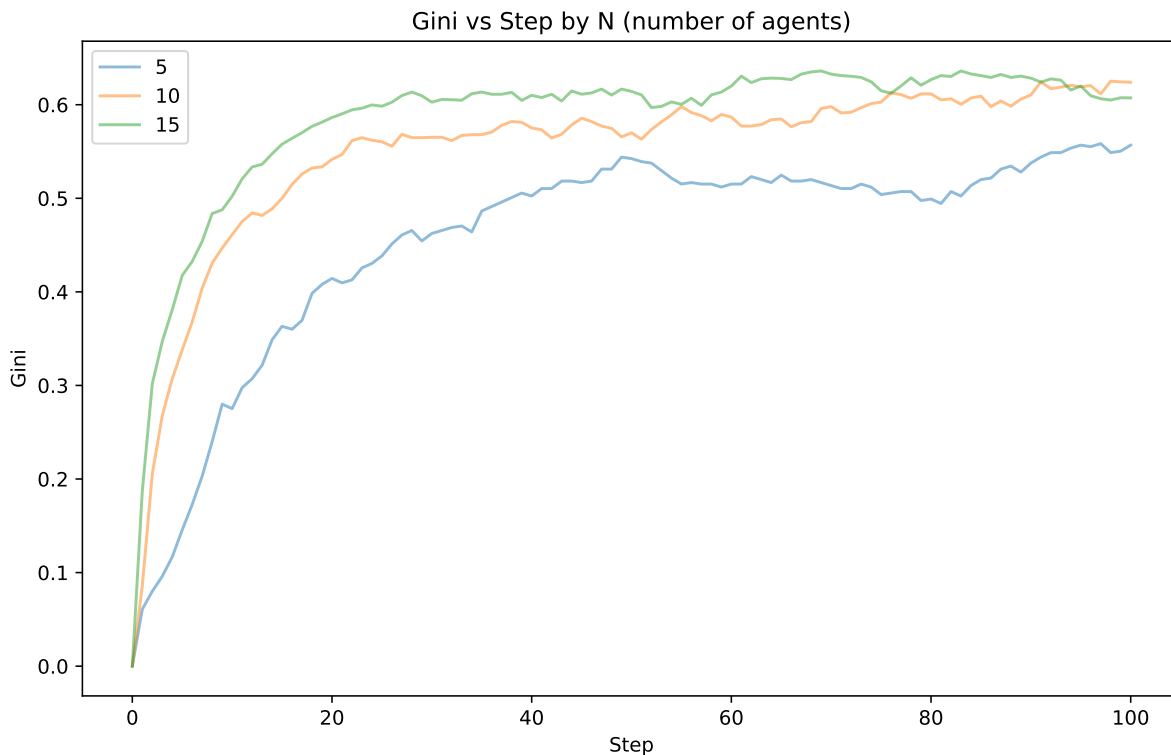
Figure 7.7: Evolution of Gini over time steps
