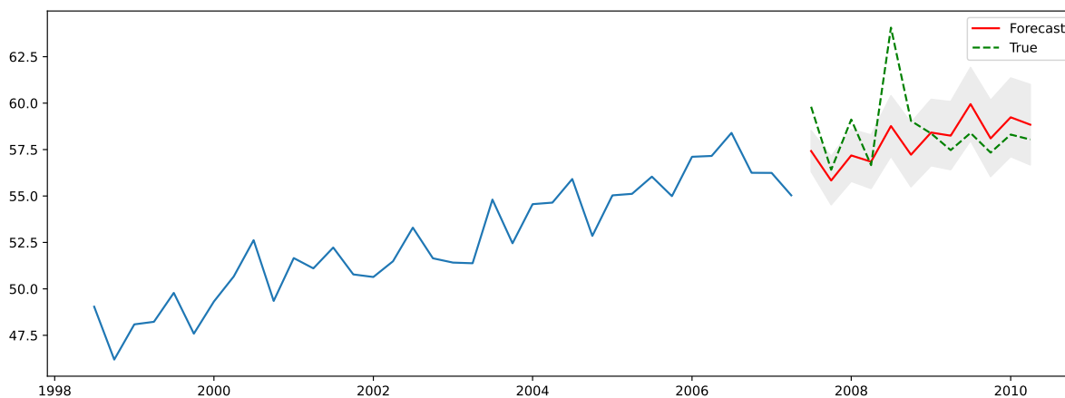
Figure 6.8: ARIMA forecasts
