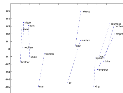
(a) GloVe
