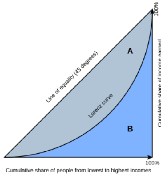
Figure 7.4: Lorenz curve
