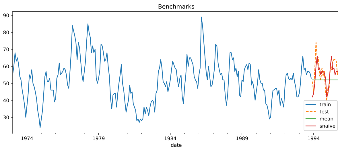
Figure 6.5: Benchmark forecasts
