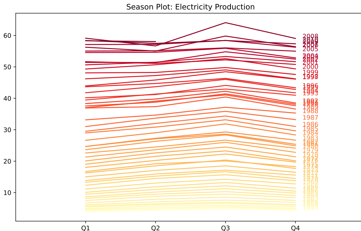
Figure 6.2: Season plot, electric production
