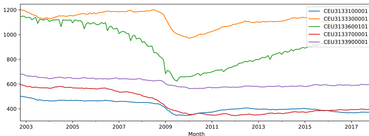
Figure 6.14: Series from top left corner of heatmap
