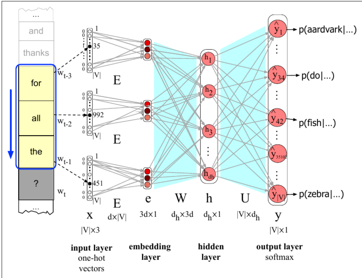
Figure 4.8: Jurafsky and Martin (2025), FFN
