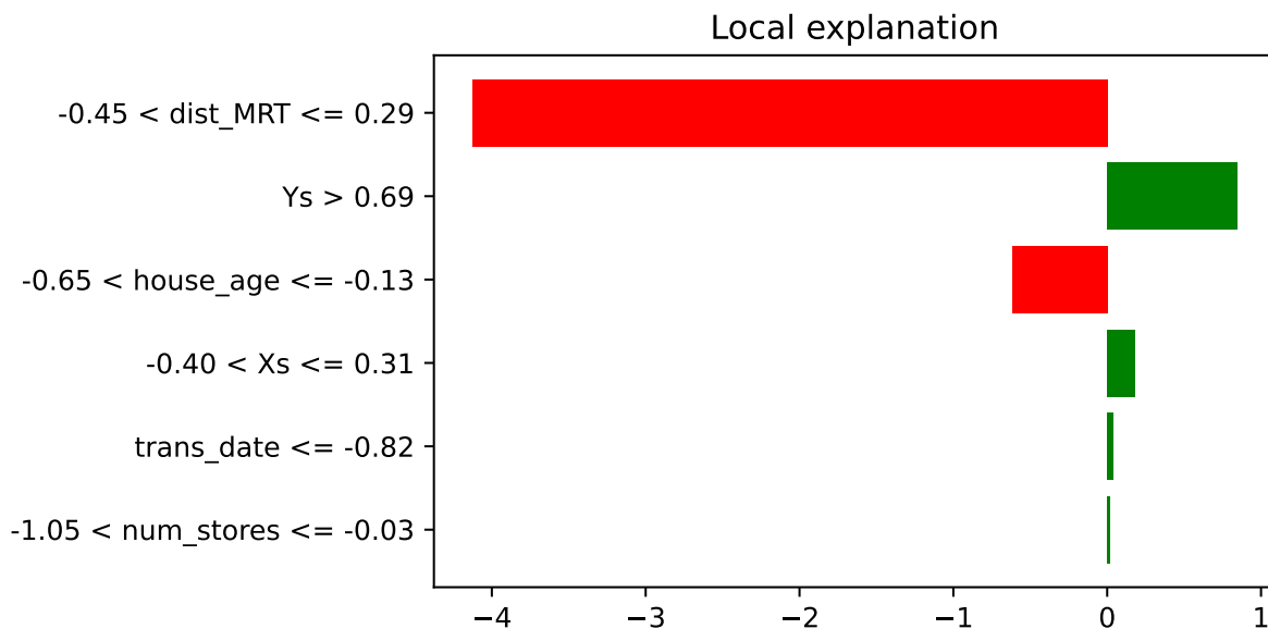
Figure 8.10: LIME Explanation for Taiwan data instance
