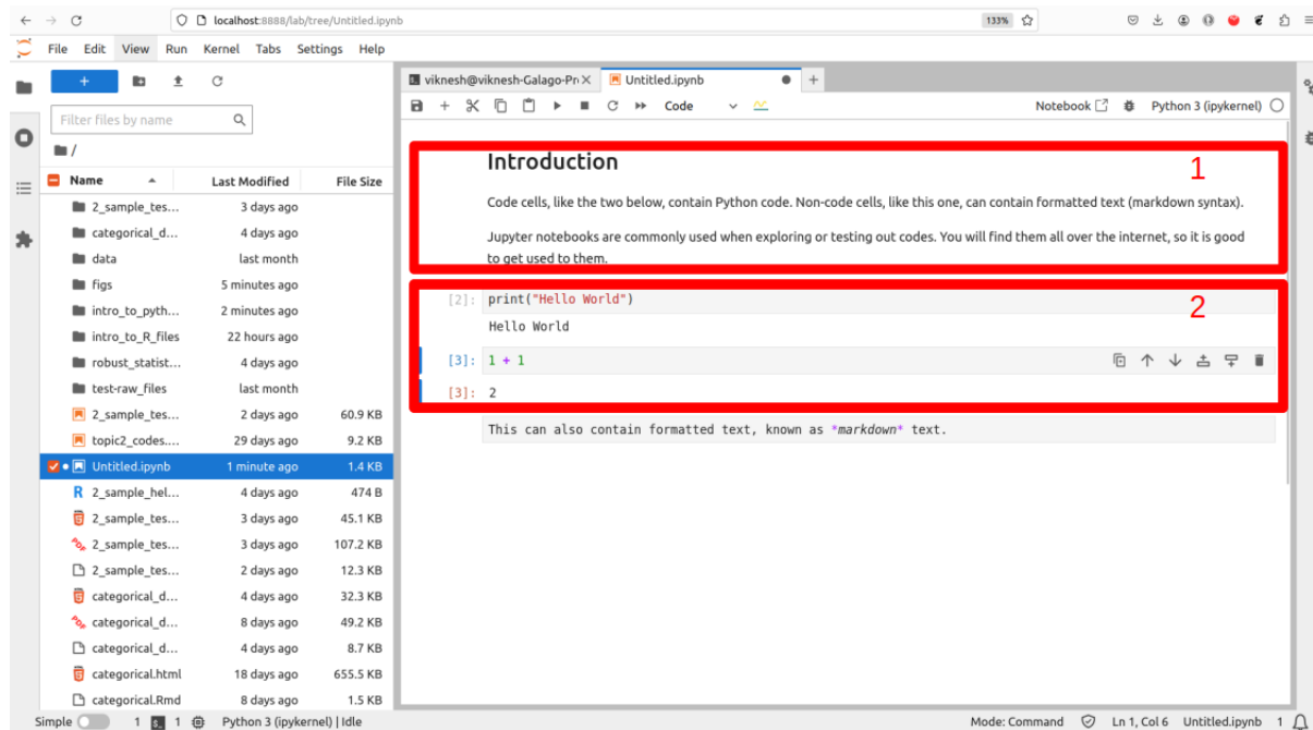
Figure 1.1: Jupyter Lab
