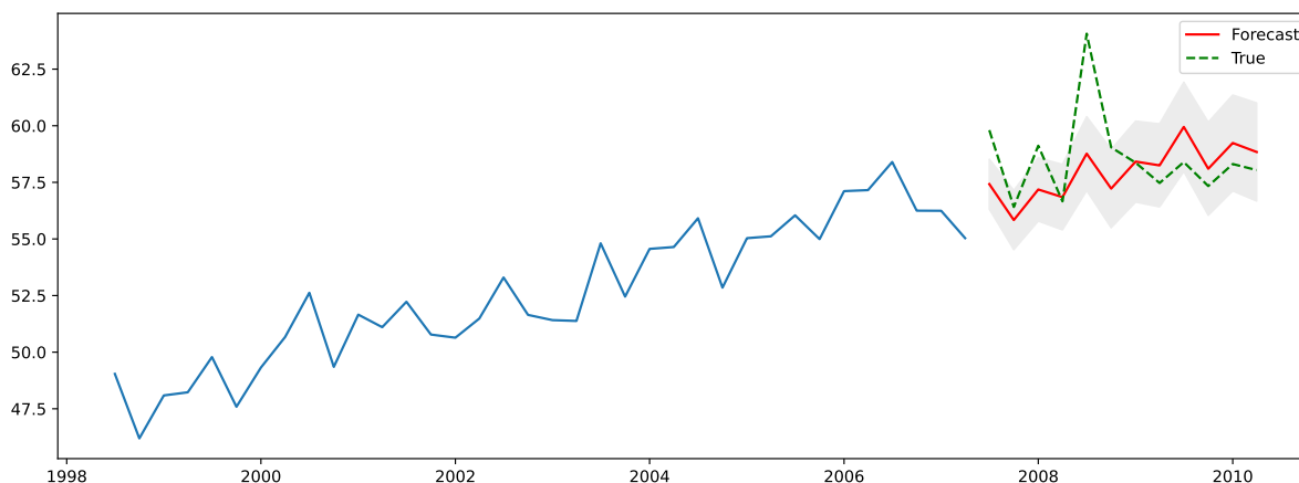
Figure 6.8: ARIMA forecasts
