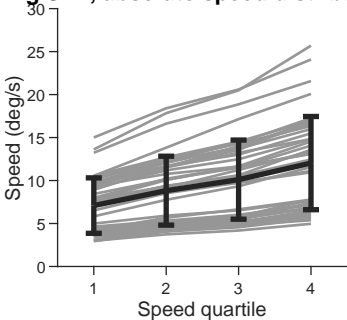
Fig S4B, absolute speed distribution
