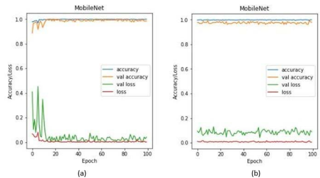
FIGURE 4. Comparison of accuracy and loss of two optimizer methods. (a) Adam, (b) SGD.
