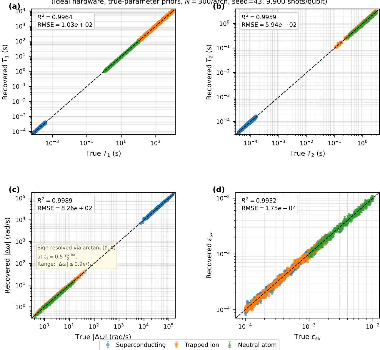
Fig. 2 — Parameter Recovery Accuracy (Ideal hardware, true-parameter priors, N = 300/\text{arch} , seed=43, 9,900 shots/qubit)
