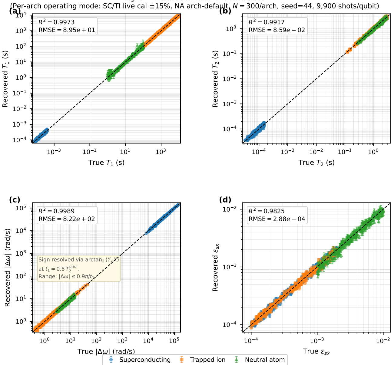
Fig. 3 — Realistic Hardware Performance
