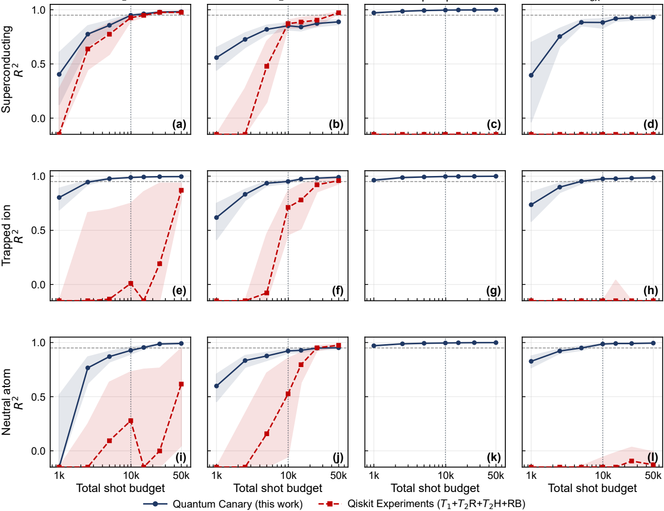
Quantum Canary vs. Qiskit Experiments — Recovery R^2 vs. Total Shot Budget
