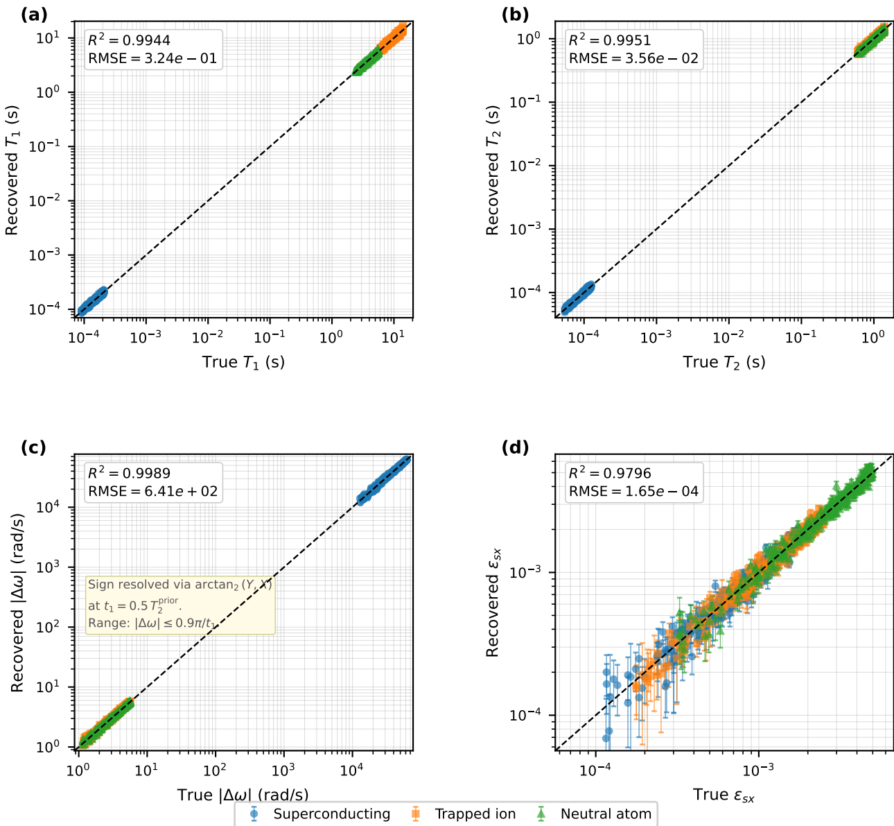
Fig. 2 — Parameter Recovery Accuracy (Digital Twin, N = 300/\text{arch} , seed=43, 9900 shots/qubit)
