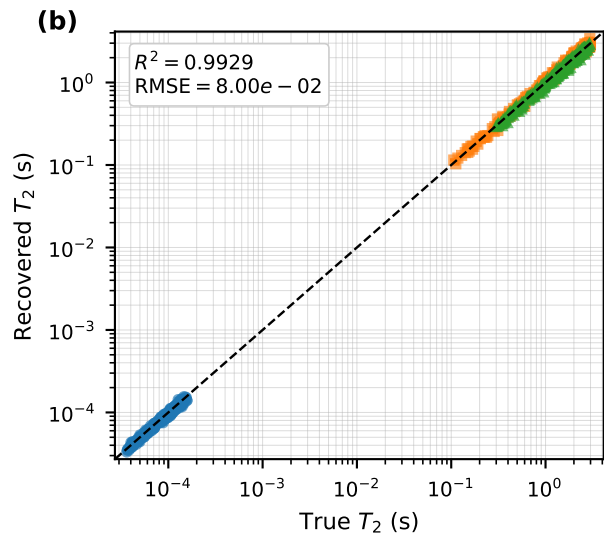
Fig. 2 — Parameter Recovery Accuracy (N=300/arch, AerSimulator, ideal Markovian)
