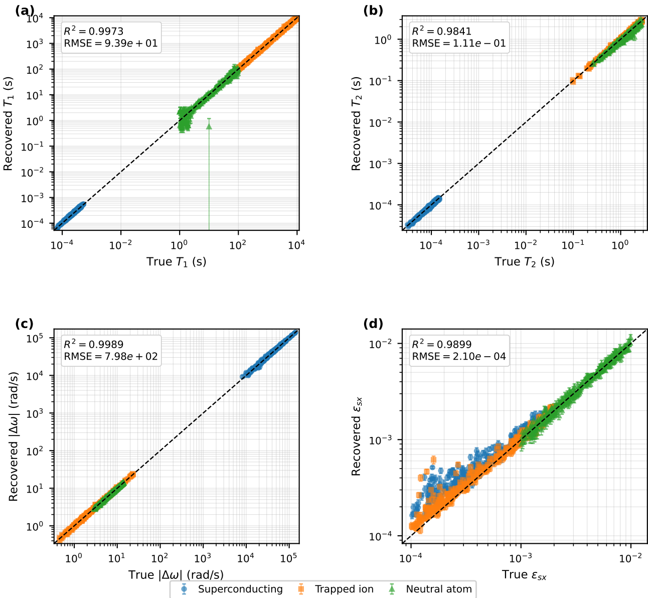
Fig. 3 — Realistic Hardware Performance (N=300/arch, unmodeled physics injected)
