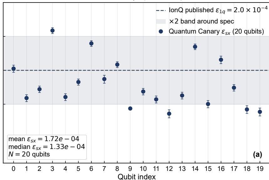
Quantum Canary \varepsilon_{SX} , all 20 qubits
