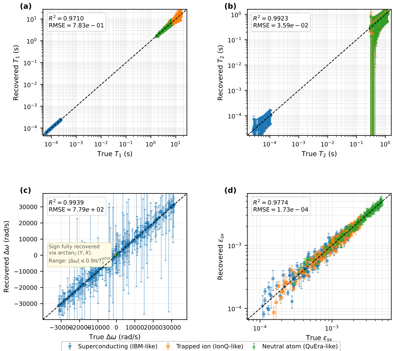
Fig. 2 — Parameter Recovery Accuracy (Digital Twin, N = 200/\text{arch} , seed=42; shots/qubit — Superconducting: 12,000, Trapped: 11,000, Neutral: 11,000)
