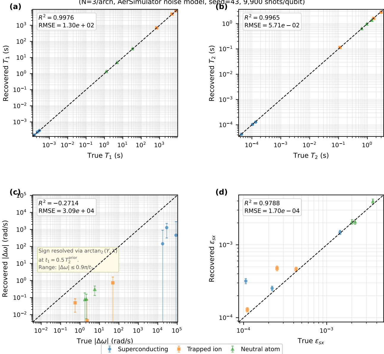
Fig. 2 — Parameter Recovery Accuracy ( N=3/\text{arch} , AerSimulator noise model, seed=43, 9,900 shots/qubit)
