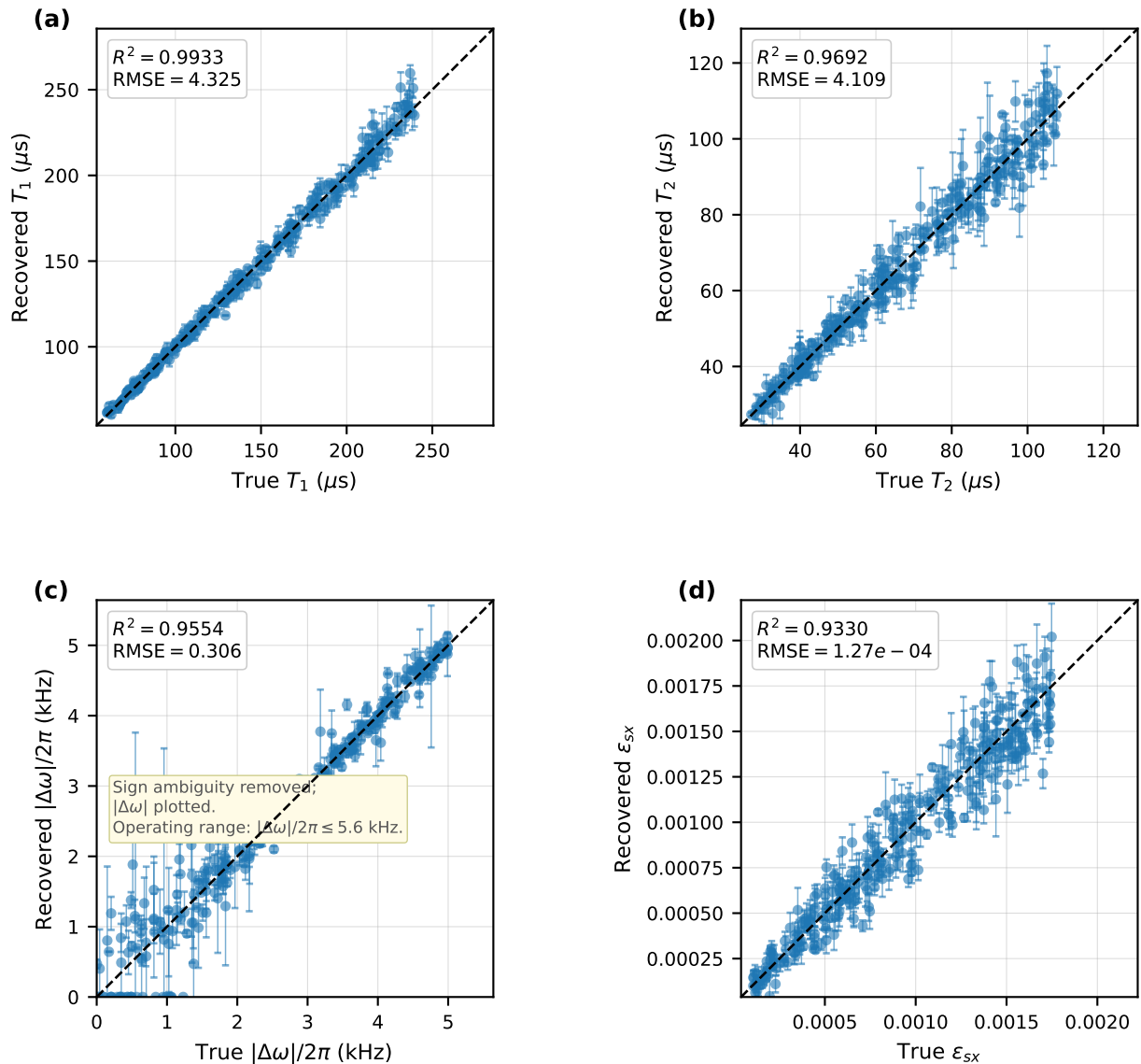
Fig. 2 — Parameter Recovery Accuracy (Digital Twin, Superconducting, N = 300 instances, 15,000 shots/qubit, seed=42)
