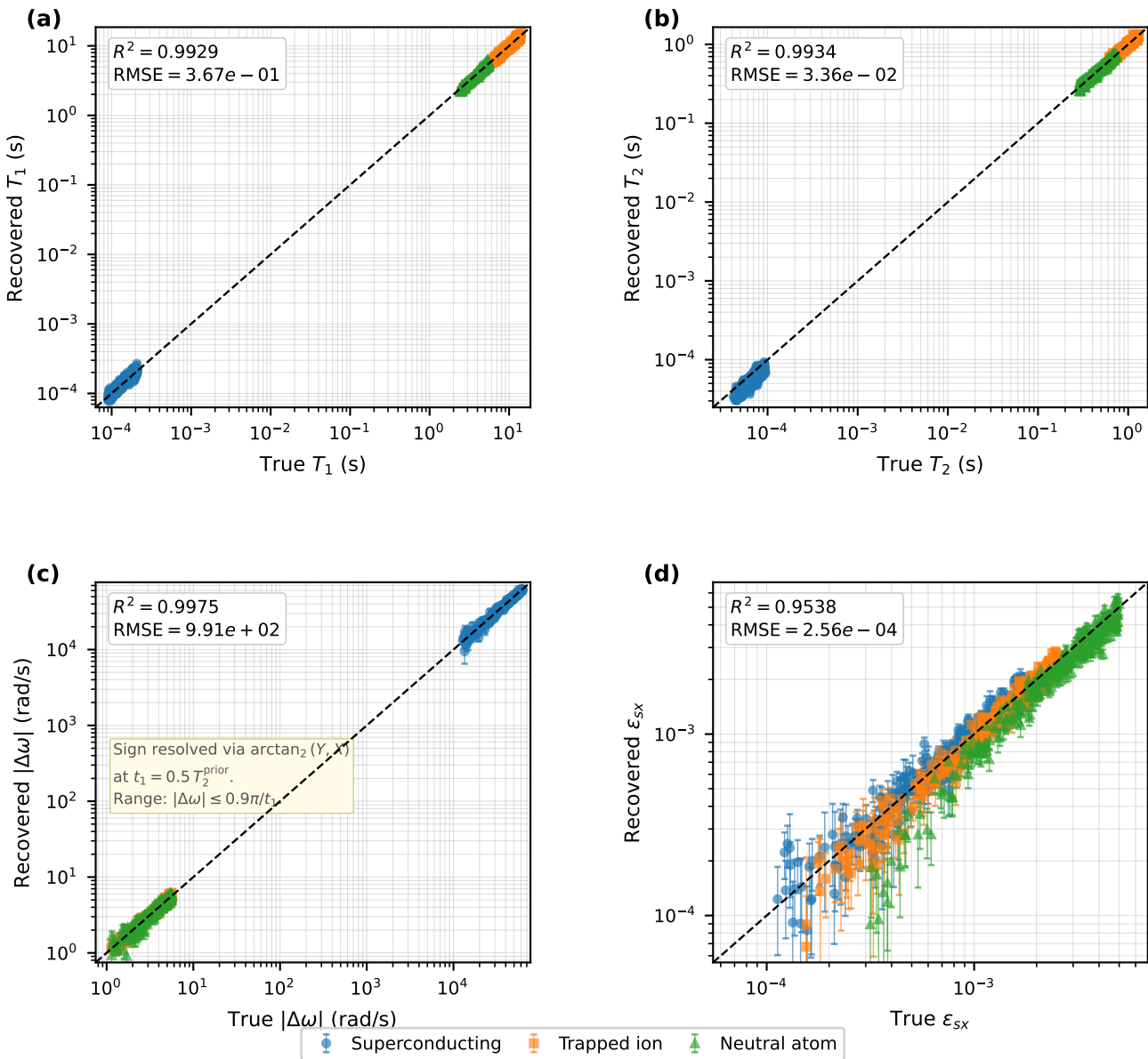
Fig. 3 — Realistic Noise Robustness (Physically Consistent, N = 300/\text{arch} , seed=44)
